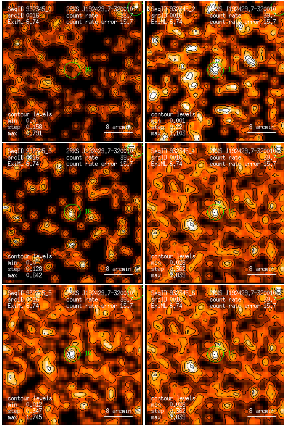
Figure 16: RASS 932345: detection 0016: band rate images, Gaussian filter: (1) PSPC channels 11 – 41, (2) 52 – 90, (3) 91 – 201, (4) 11 – 235, (5) 52 – 201, (6) 11 – 201. Broad band rates in counts/ks. Band rate contour levels in counts/ks/arcmin 2 .
