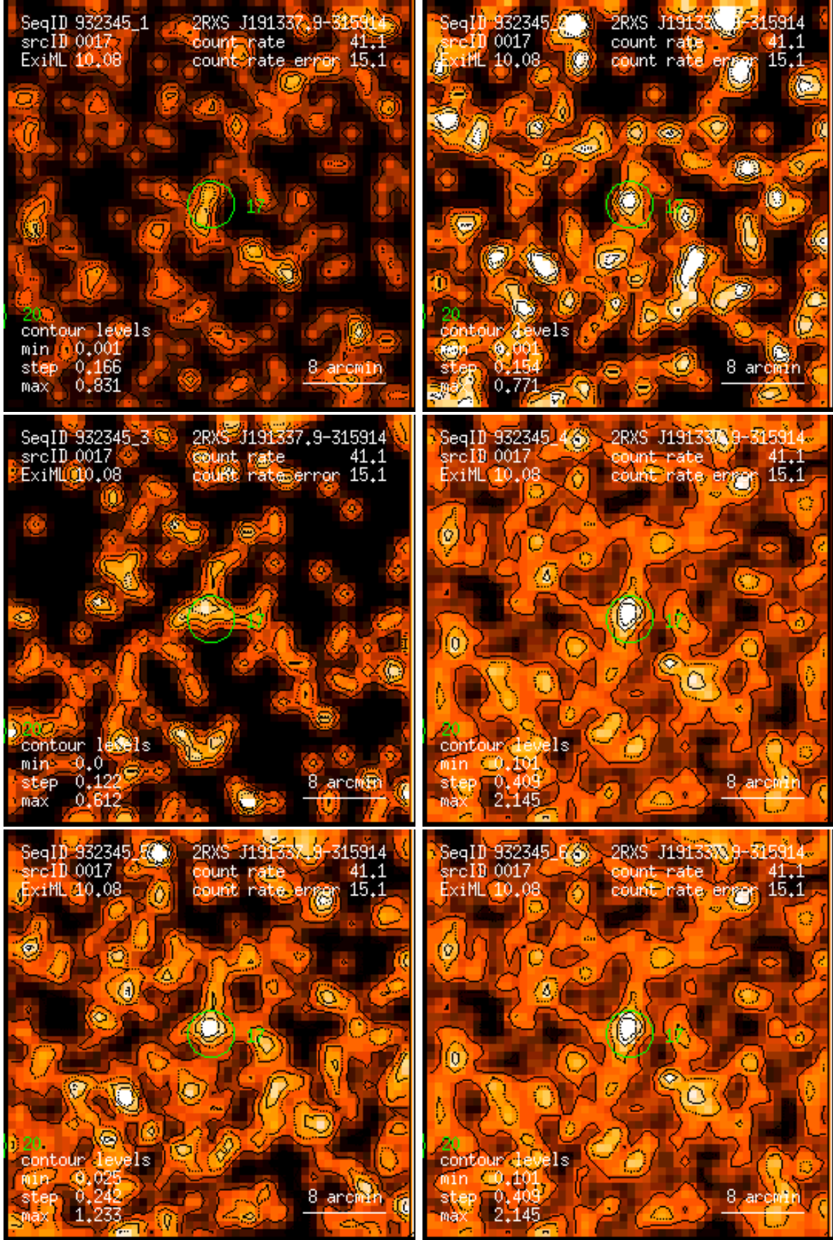
Figure 17: RASS 932345: detection 0017: band rate images, Gaussian filter: (1) PSPC channels 11 – 41, (2) 52 – 90, (3) 91 – 201, (4) 11 – 235, (5) 52 – 201, (6) 11 – 201. Broad band rates in counts/ks. Band rate contour levels in counts/ks/arcmin 2 .
