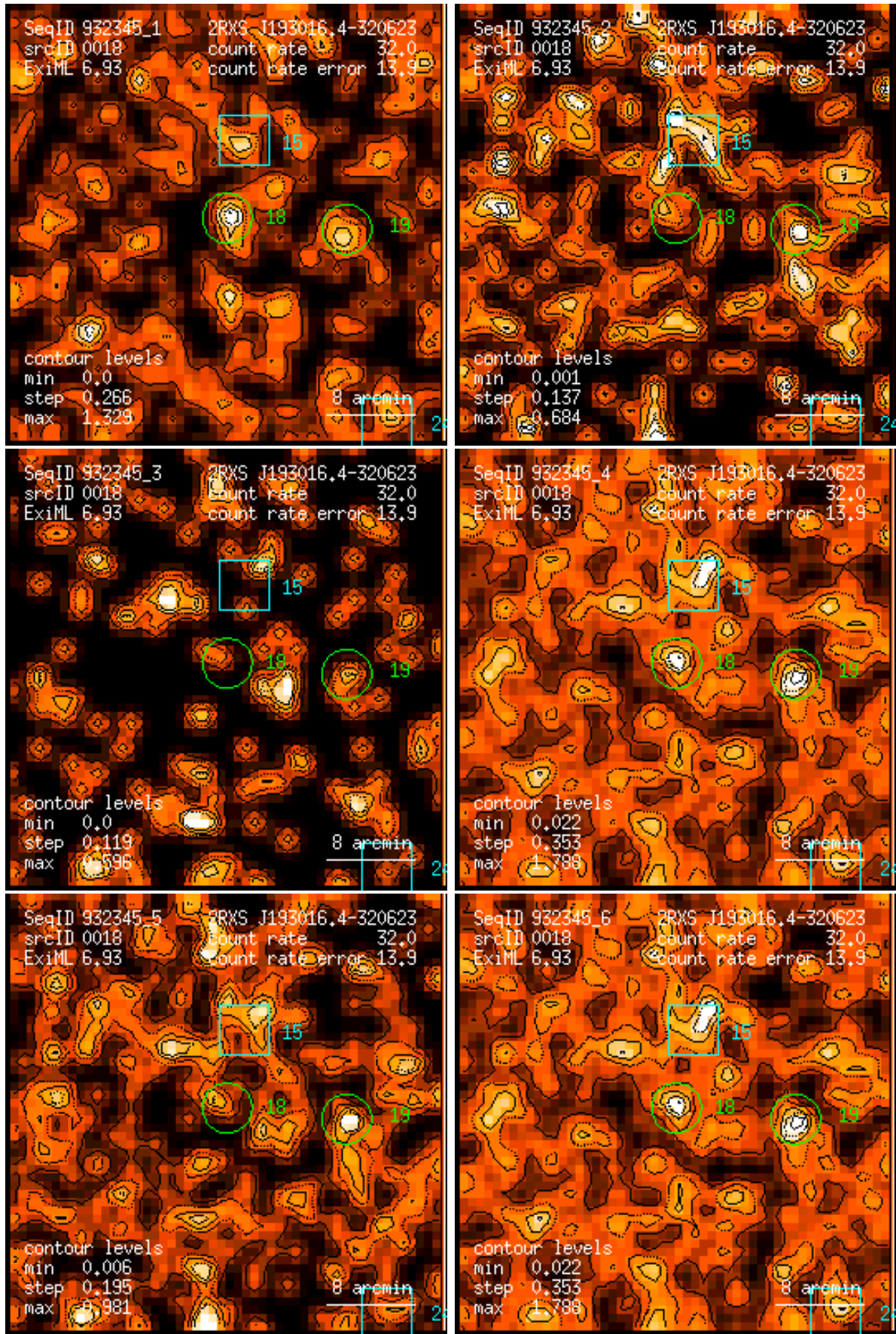
Figure 18: RASS 932345: detection 0018: band rate images, Gaussian filter: (1) PSPC channels 11 – 41, (2) 52 – 90, (3) 91 – 201, (4) 11 – 235, (5) 52 – 201, (6) 11 – 201. Broad band rates in counts/ks. Band rate contour levels in counts/ks/arcmin 2 .
