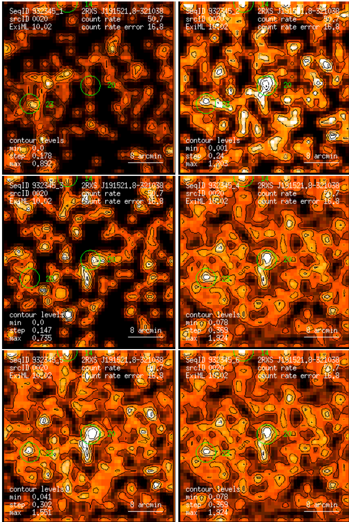
Figure 20: RASS 932345: detection 0020: band rate images, Gaussian filter: (1) PSPC channels 11 – 41, (2) 52 – 90, (3) 91 – 201, (4) 11 – 235, (5) 52 – 201, (6) 11 – 201. Broad band rates in counts/ks. Band rate contour levels in counts/ks/arcmin 2 .
