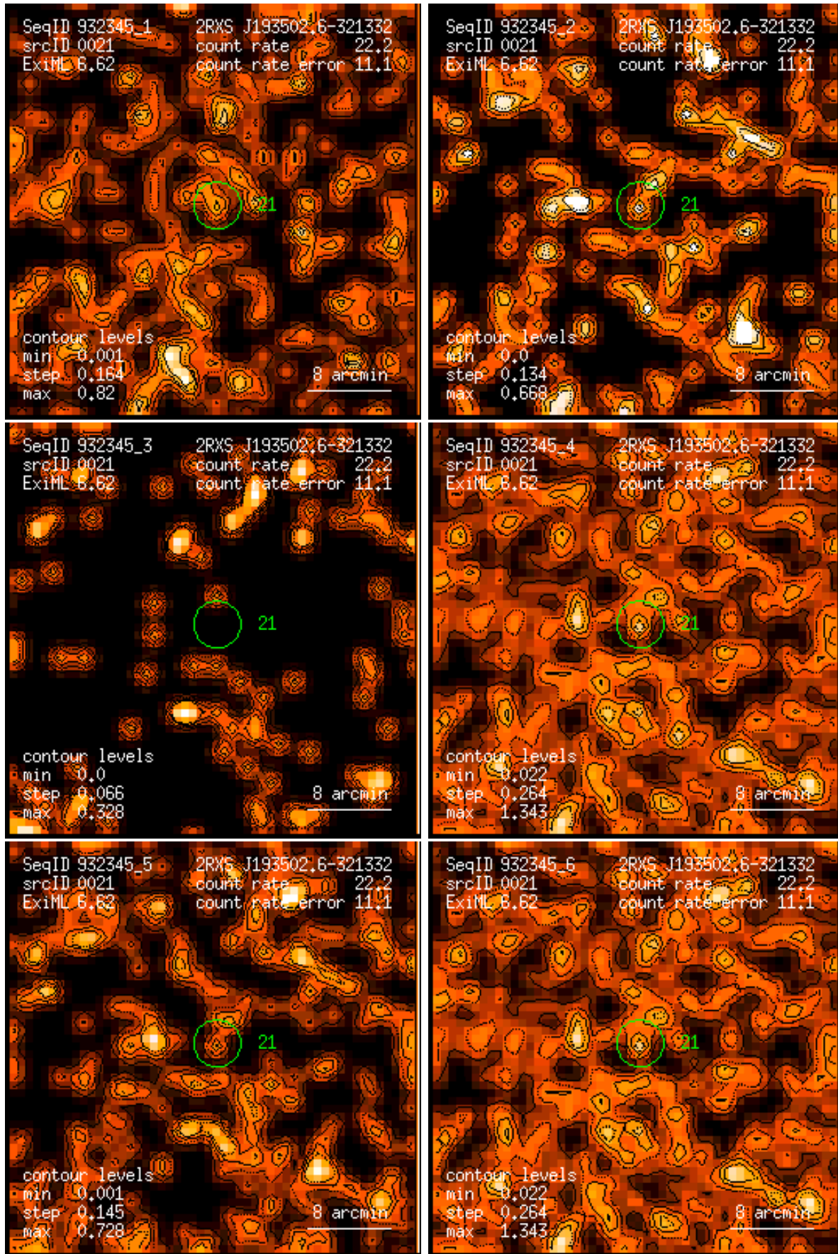
Figure 21: RASS 932345: detection 0021: band rate images, Gaussian filter: (1) PSPC channels 11 – 41, (2) 52 – 90, (3) 91 – 201, (4) 11 – 235, (5) 52 – 201, (6) 11 – 201. Broad band rates in counts/ks. Band rate contour levels in counts/ks/arcmin 2 .
