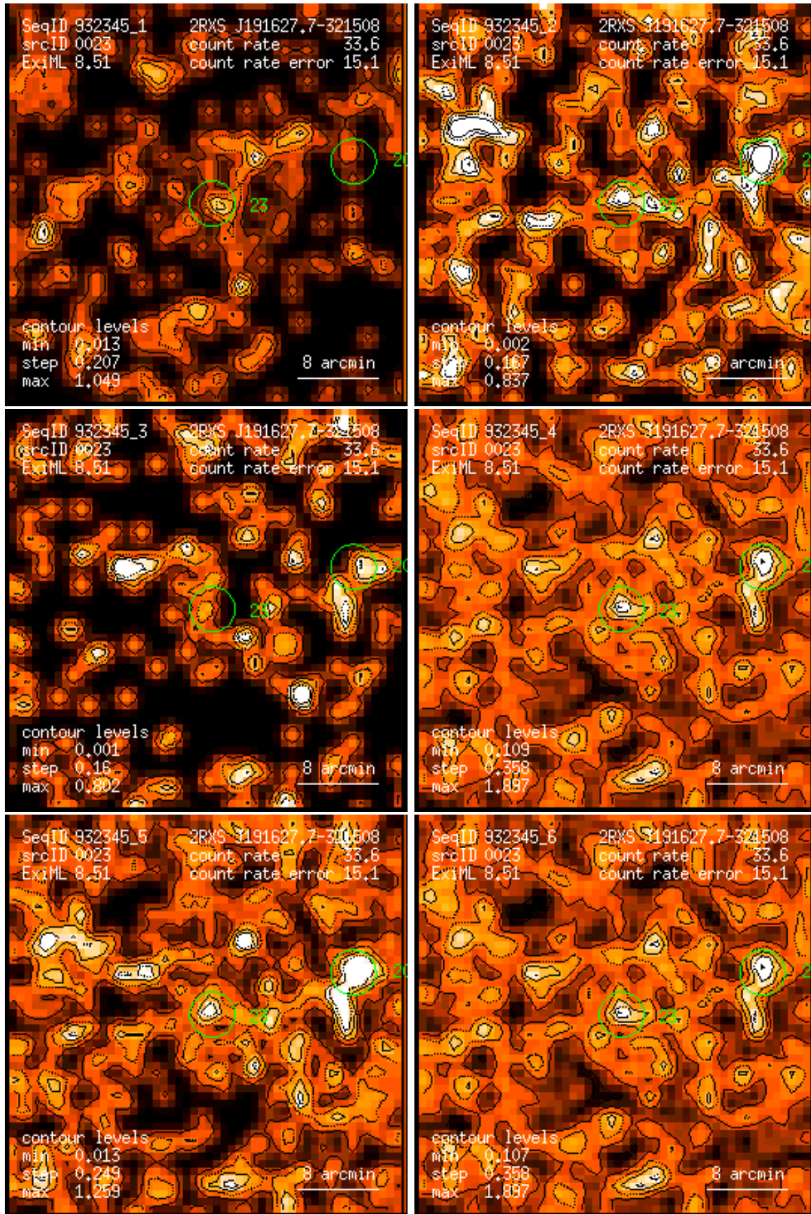
Figure 23: RASS 932345: detection 0023: band rate images, Gaussian filter: (1) PSPC channels 11 – 41, (2) 52 – 90, (3) 91 – 201, (4) 11 – 235, (5) 52 – 201, (6) 11 – 201. Broad band rates in counts/ks. Band rate contour levels in counts/ks/arcmin 2 .
