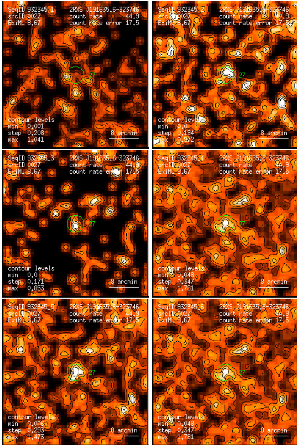
Figure 27: RASS 932345: detection 0027: band rate images, Gaussian filter: (1) PSPC channels 11 – 41, (2) 52 – 90, (3) 91 – 201, (4) 11 – 235, (5) 52 – 201, (6) 11 – 201. Broad band rates in counts/ks. Band rate contour levels in counts/ks/arcmin 2 .
