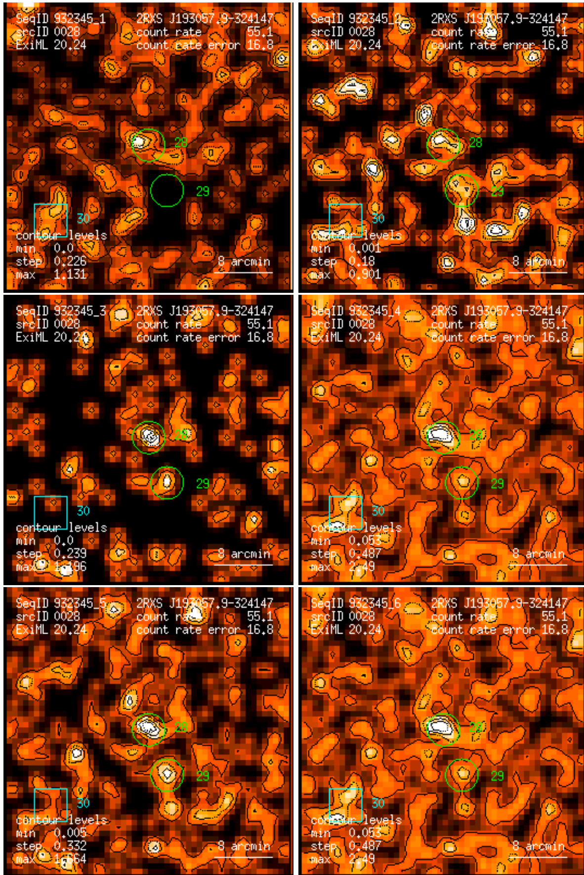
Figure 28: RASS 932345: detection 0028: band rate images, Gaussian filter: (1) PSPC channels 11 – 41, (2) 52 – 90, (3) 91 – 201, (4) 11 – 235, (5) 52 – 201, (6) 11 – 201. Broad band rates in counts/ks. Band rate contour levels in counts/ks/arcmin 2 .
