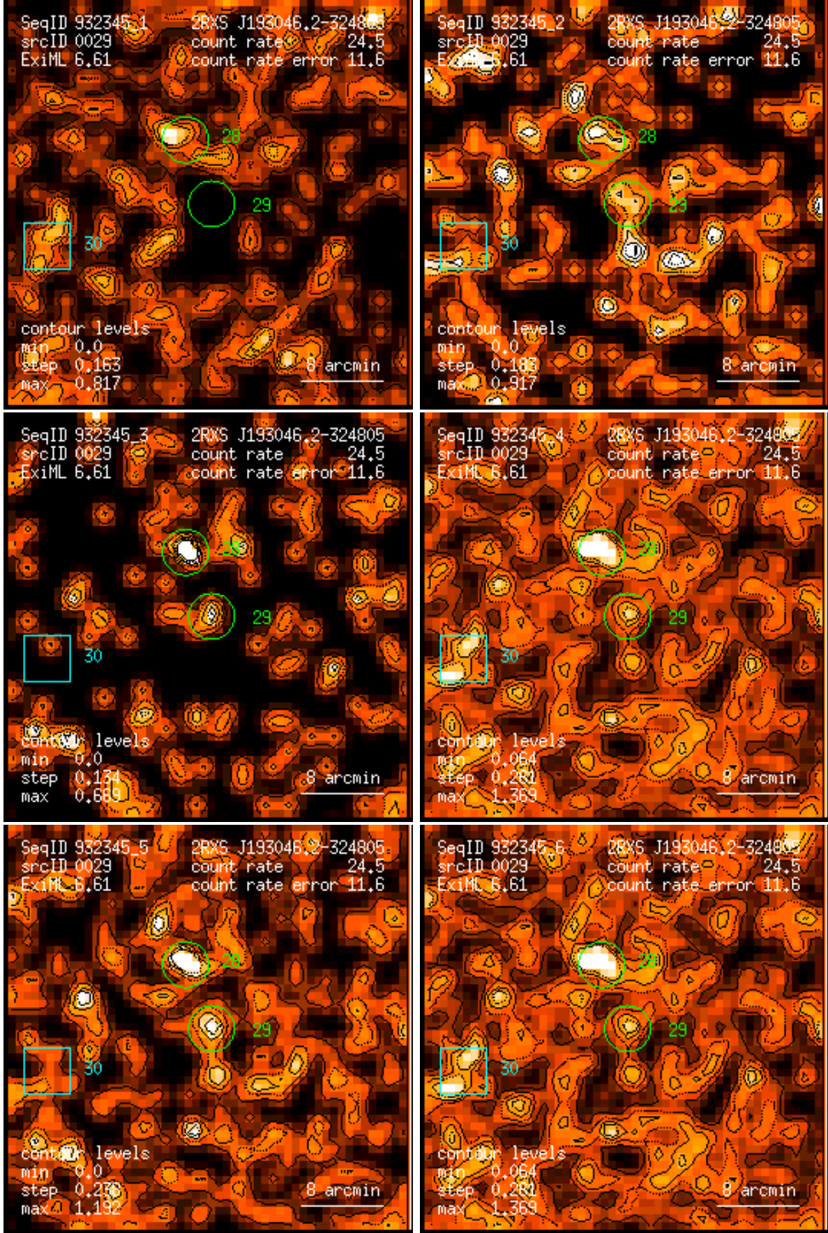
Figure 29: RASS 932345: detection 0029: band rate images, Gaussian filter: (1) PSPC channels 11 – 41, (2) 52 – 90, (3) 91 – 201, (4) 11 – 235, (5) 52 – 201, (6) 11 – 201. Broad band rates in counts/ks. Band rate contour levels in counts/ks/arcmin 2 .
