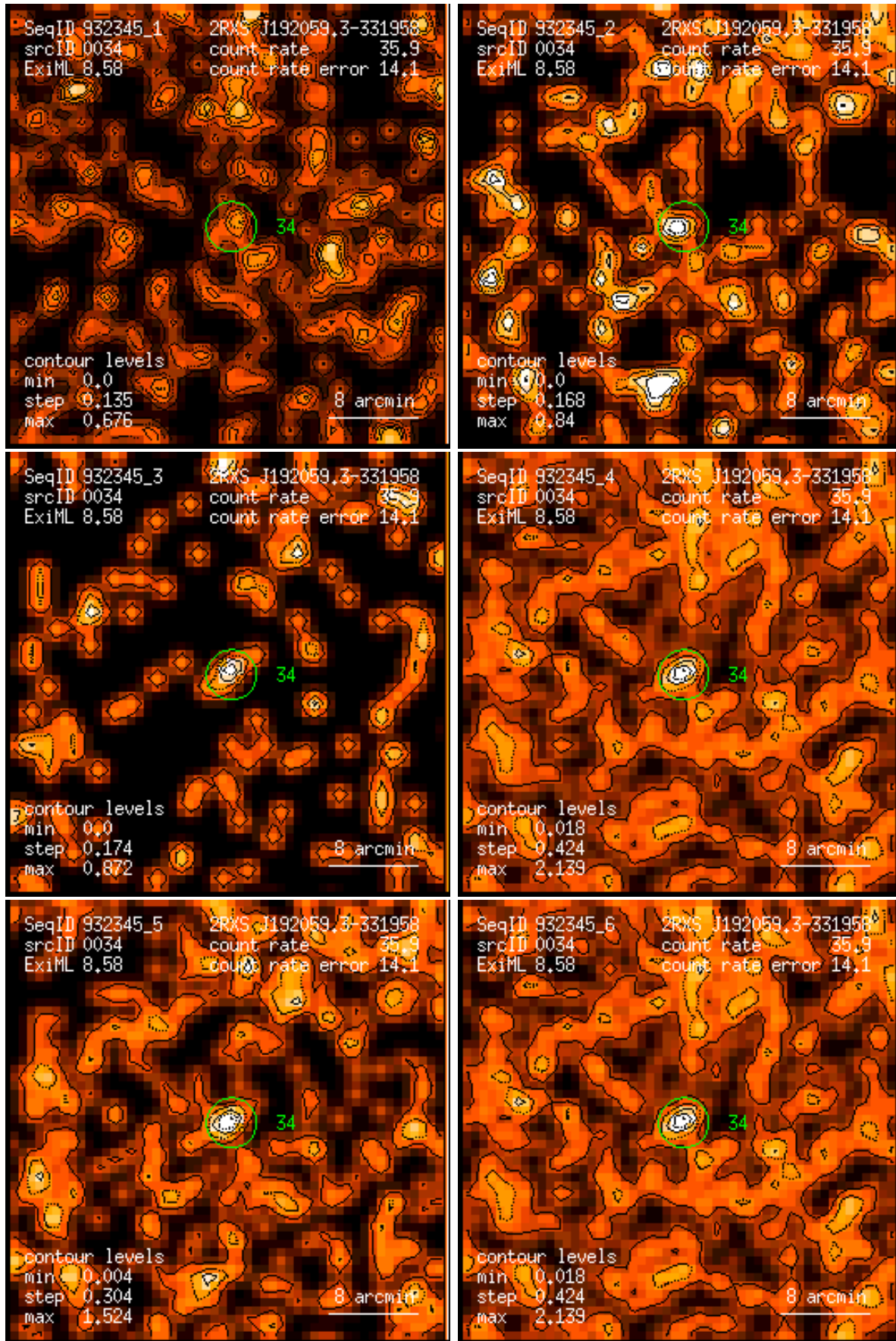
Figure 34: RASS 932345: detection 0034: band rate images, Gaussian filter: (1) PSPC channels 11 – 41, (2) 52 – 90, (3) 91 – 201, (4) 11 – 235, (5) 52 – 201, (6) 11 – 201. Broad band rates in counts/ks. Band rate contour levels in counts/ks/arcmin 2 .
