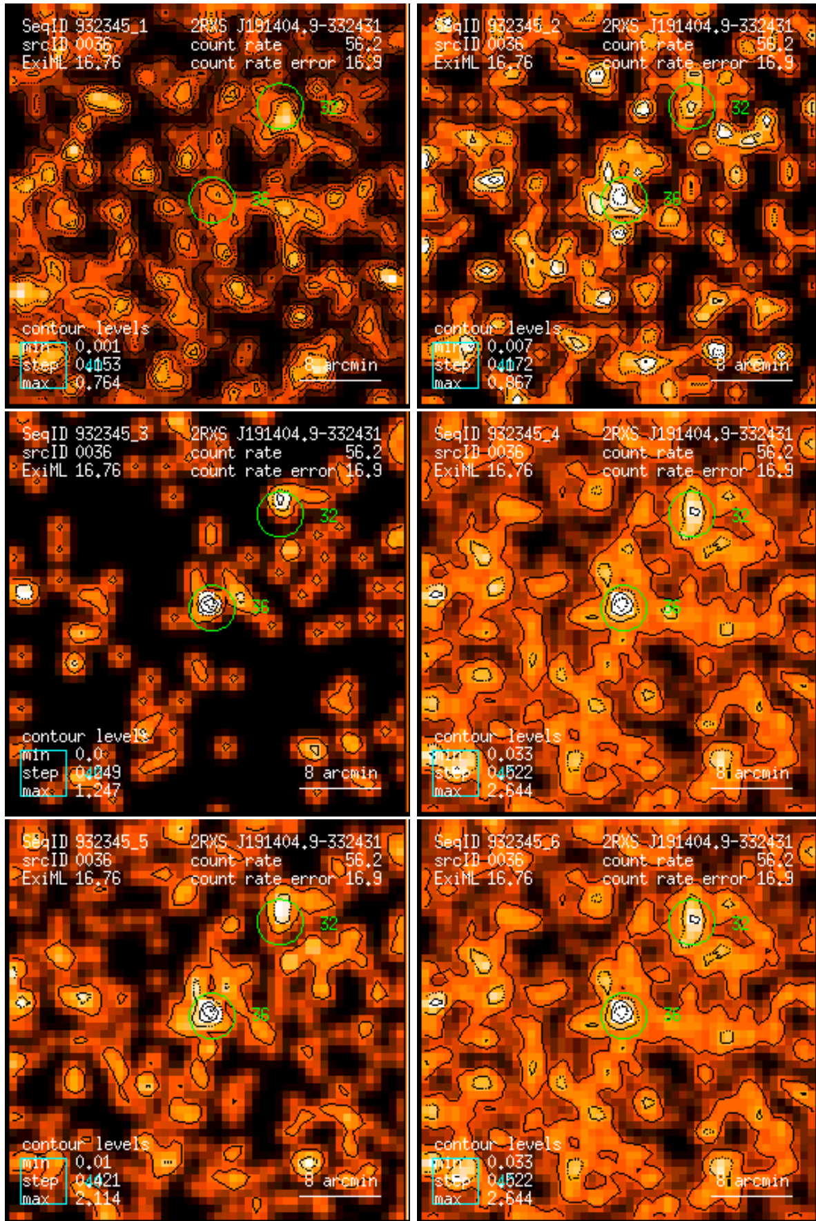
Figure 36: RASS 932345: detection 0036: band rate images, Gaussian filter: (1) PSPC channels 11 – 41, (2) 52 – 90, (3) 91 – 201, (4) 11 – 235, (5) 52 – 201, (6) 11 – 201. Broad band rates in counts/ks. Band rate contour levels in counts/ks/arcmin 2 .
