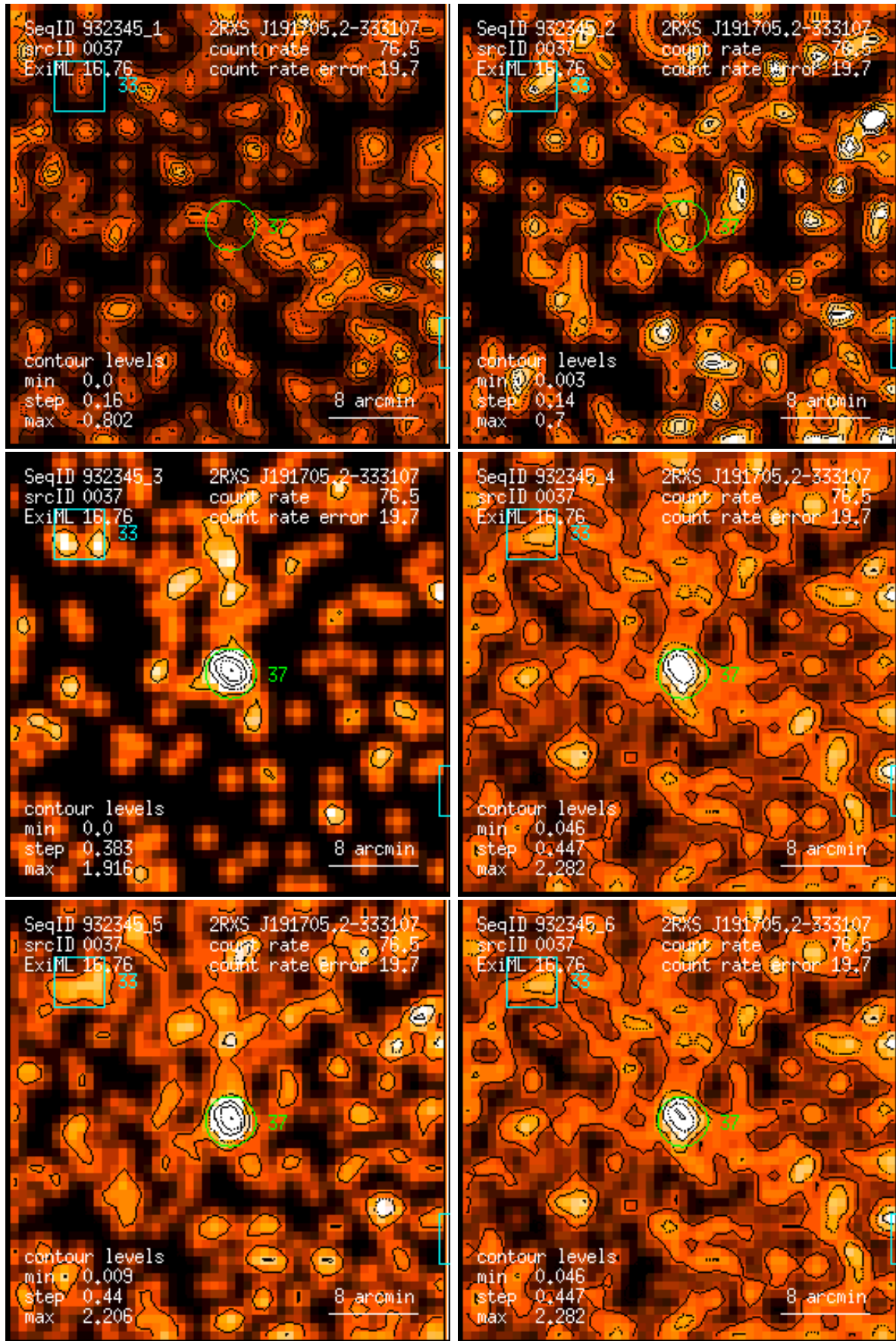
Figure 37: RASS 932345: detection 0037: band rate images, Gaussian filter: (1) PSPC channels 11 – 41, (2) 52 – 90, (3) 91 – 201, (4) 11 – 235, (5) 52 – 201, (6) 11 – 201. Broad band rates in counts/ks. Band rate contour levels in counts/ks/arcmin 2 .
