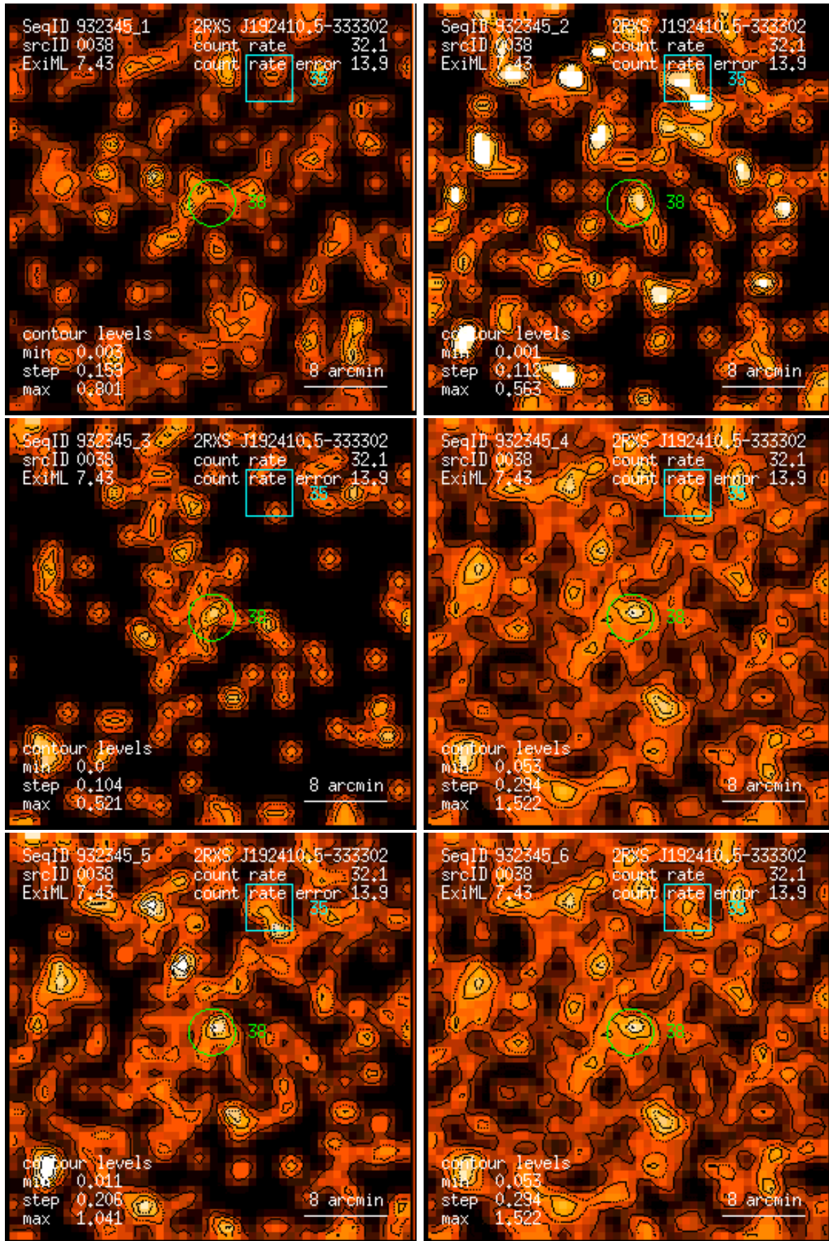
Figure 38: RASS 932345: detection 0038: band rate images, Gaussian filter: (1) PSPC channels 11 – 41, (2) 52 – 90, (3) 91 – 201, (4) 11 – 235, (5) 52 – 201, (6) 11 – 201. Broad band rates in counts/ks. Band rate contour levels in counts/ks/arcmin 2 .
