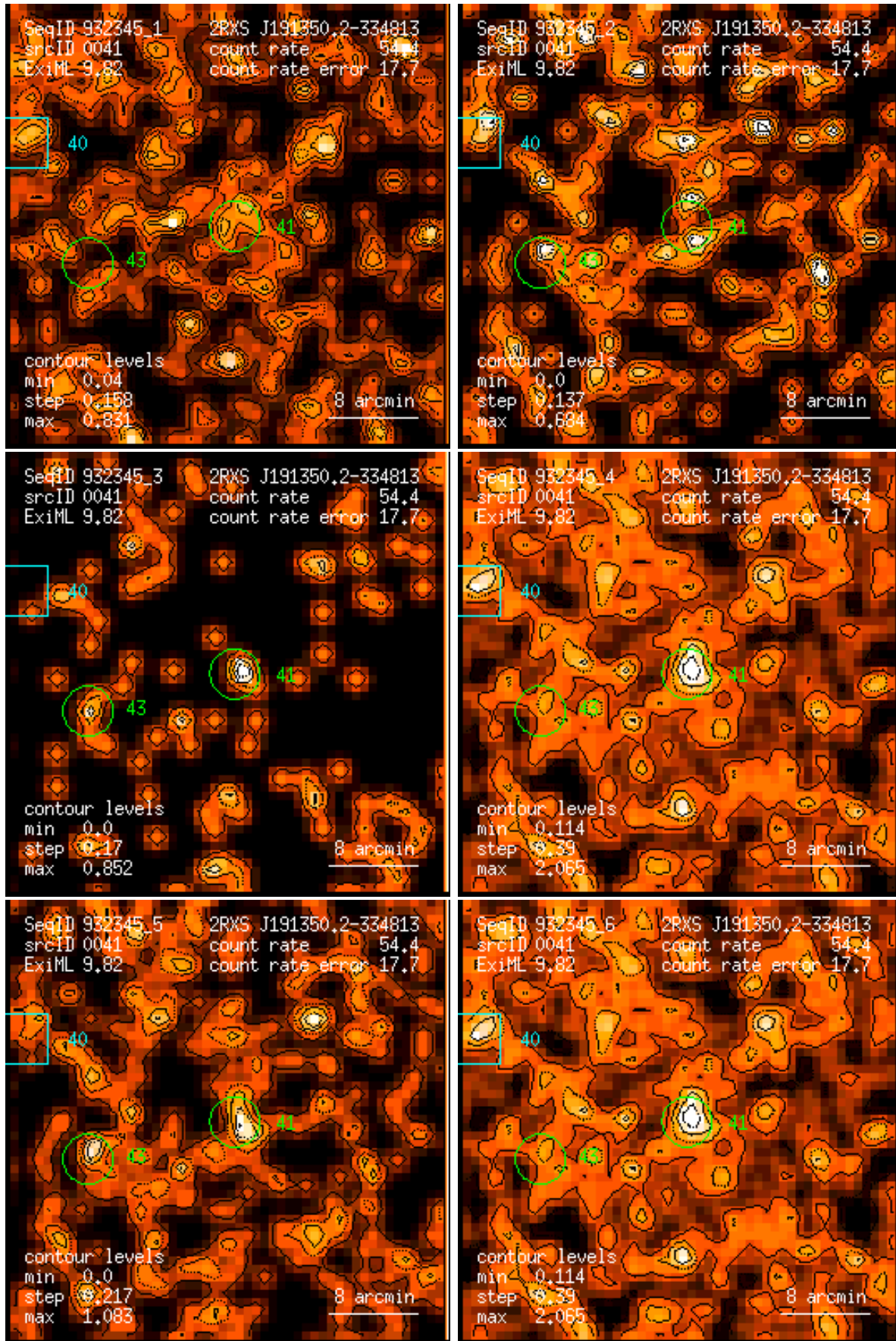
Figure 41: RASS 932345: detection 0041: band rate images, Gaussian filter: (1) PSPC channels 11 – 41, (2) 52 – 90, (3) 91 – 201, (4) 11 – 235, (5) 52 – 201, (6) 11 – 201. Broad band rates in counts/ks. Band rate contour levels in counts/ks/arcmin 2 .
