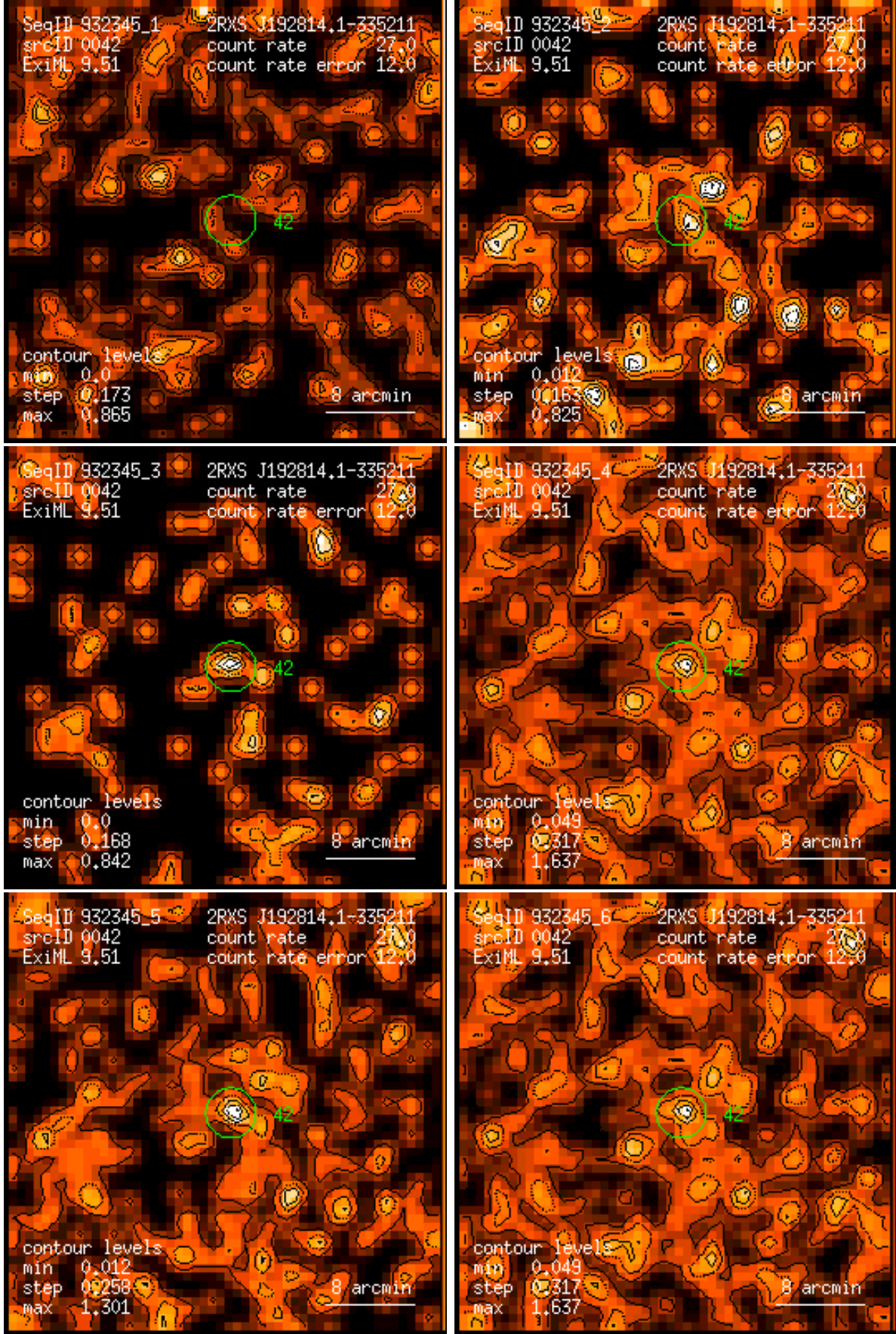
Figure 42: RASS 932345: detection 0042: band rate images, Gaussian filter: (1) PSPC channels 11 – 41, (2) 52 – 90, (3) 91 – 201, (4) 11 – 235, (5) 52 – 201, (6) 11 – 201. Broad band rates in counts/ks. Band rate contour levels in counts/ks/arcmin 2 .
