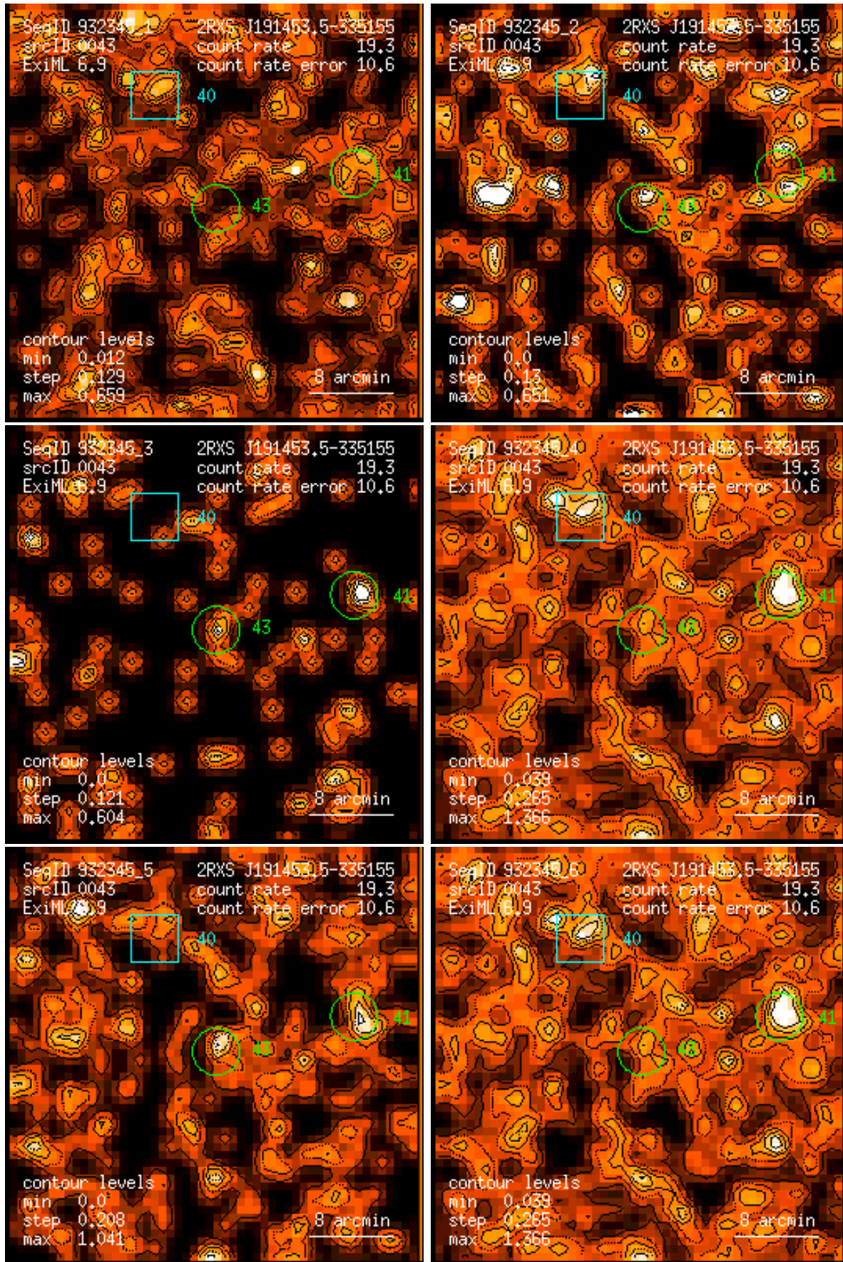
Figure 43: RASS 932345: detection 0043: band rate images, Gaussian filter: (1) PSPC channels 11 – 41, (2) 52 – 90, (3) 91 – 201, (4) 11 – 235, (5) 52 – 201, (6) 11 – 201. Broad band rates in counts/ks. Band rate contour levels in counts/ks/arcmin 2 .
