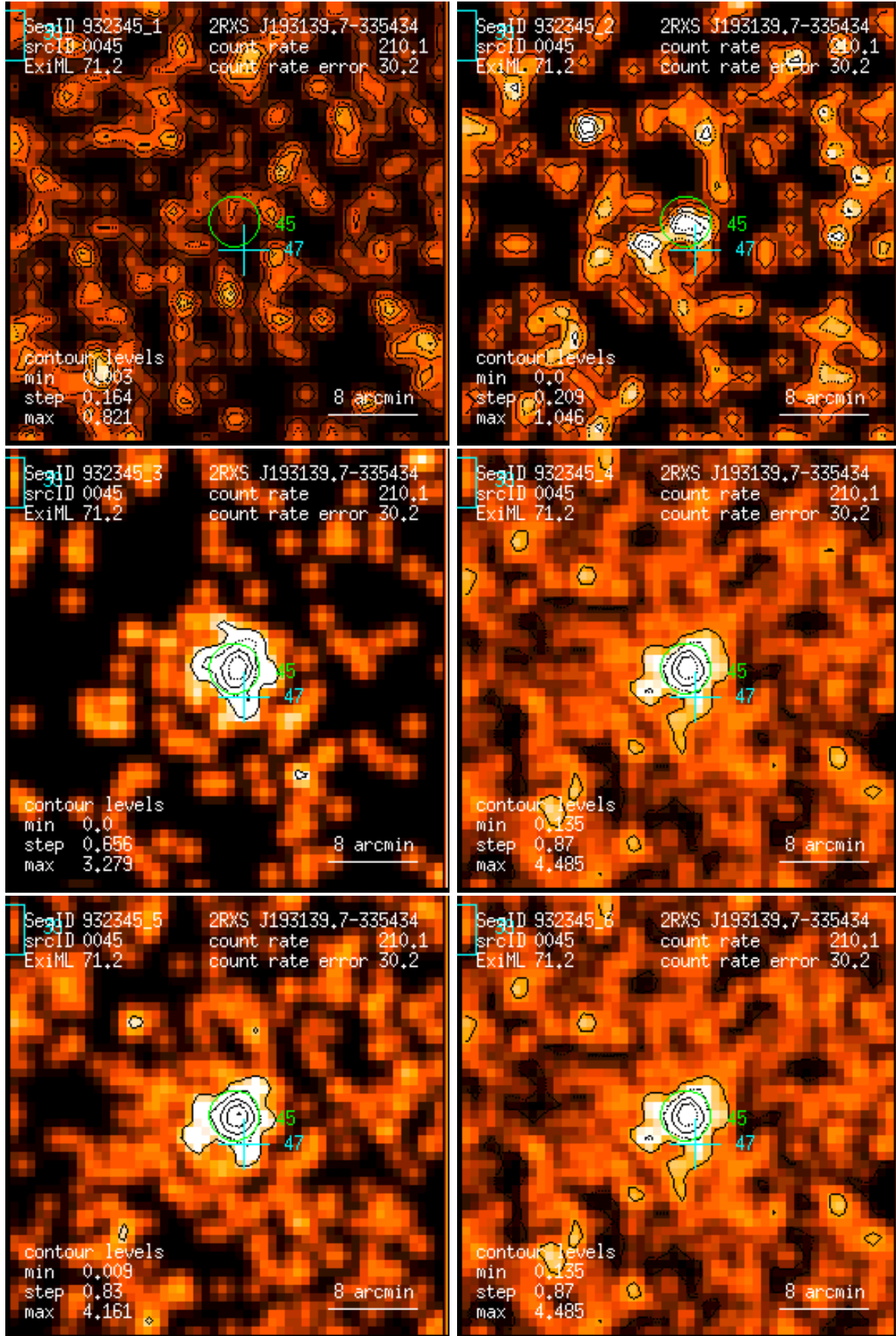
Figure 45: RASS 932345: detection 0045: band rate images, Gaussian filter: (1) PSPC channels 11 – 41, (2) 52 – 90, (3) 91 – 201, (4) 11 – 235, (5) 52 – 201, (6) 11 – 201. Broad band rates in counts/ks. Band rate contour levels in counts/ks/arcmin 2 .
