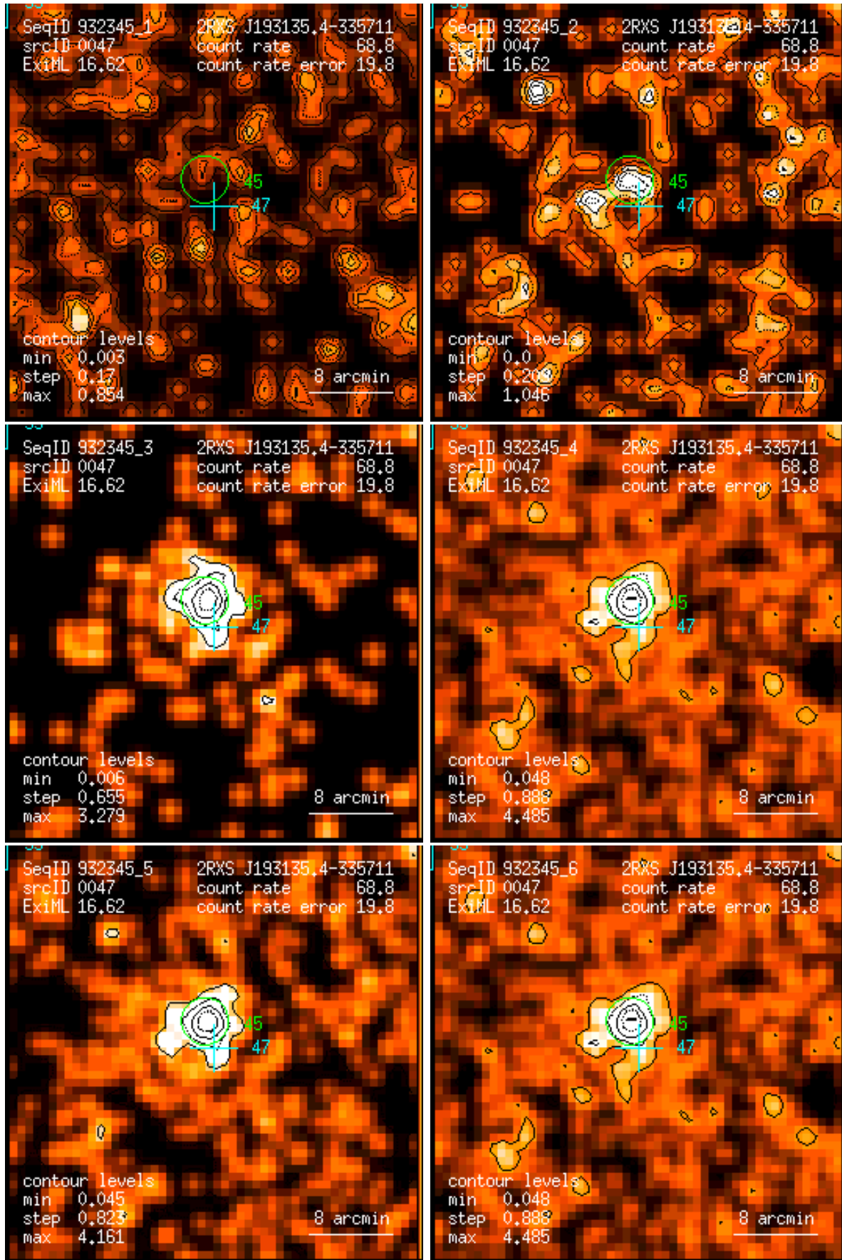
Figure 47: RASS 932345: detection 0047: band rate images, Gaussian filter: (1) PSPC channels 11 – 41, (2) 52 – 90, (3) 91 – 201, (4) 11 – 235, (5) 52 – 201, (6) 11 – 201. Broad band rates in counts/ks. Band rate contour levels in counts/ks/arcmin 2 .
