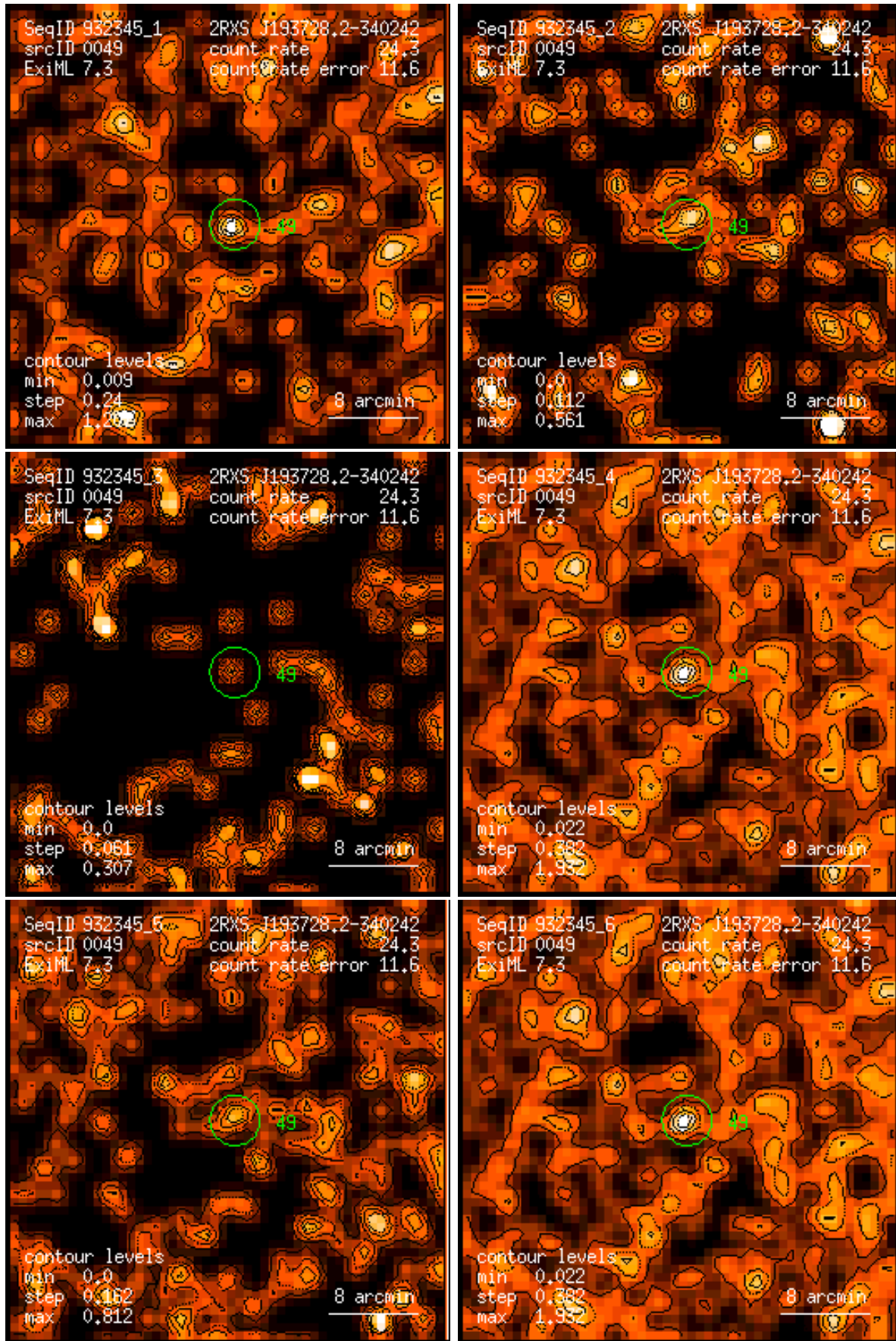
Figure 49: RASS 932345: detection 0049: band rate images, Gaussian filter: (1) PSPC channels 11 – 41, (2) 52 – 90, (3) 91 – 201, (4) 11 – 235, (5) 52 – 201, (6) 11 – 201. Broad band rates in counts/ks. Band rate contour levels in counts/ks/arcmin 2 .
