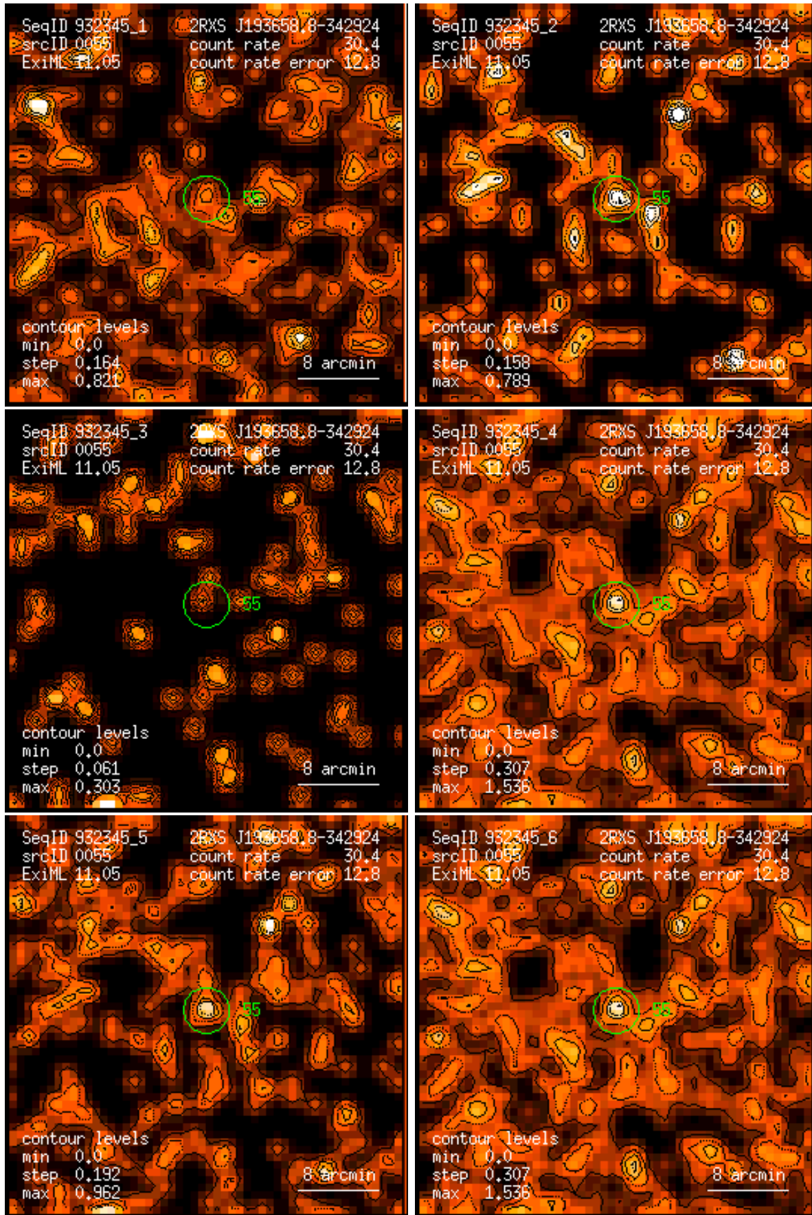
Figure 55: RASS 932345: detection 0055: band rate images, Gaussian filter: (1) PSPC channels 11 – 41, (2) 52 – 90, (3) 91 – 201, (4) 11 – 235, (5) 52 – 201, (6) 11 – 201. Broad band rates in counts/ks. Band rate contour levels in counts/ks/arcmin 2 .
