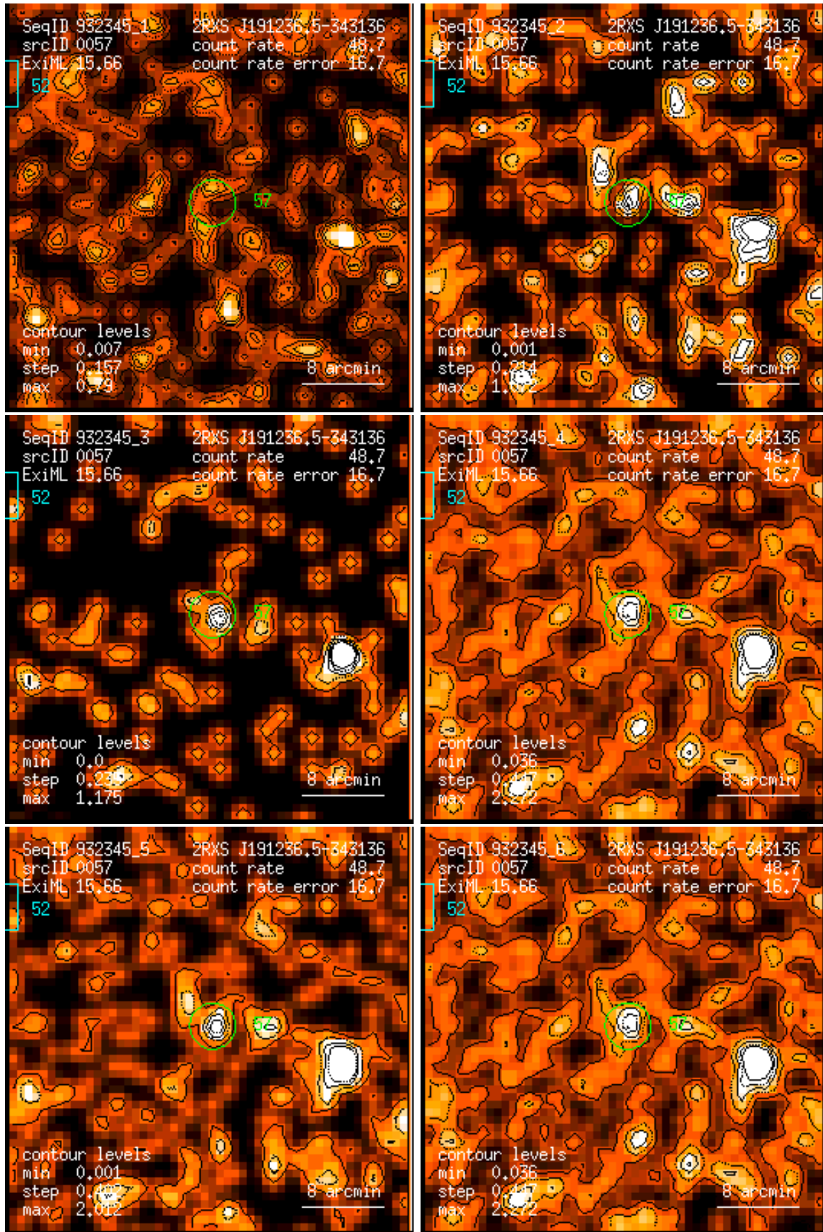
Figure 57: RASS 932345: detection 0057: band rate images, Gaussian filter: (1) PSPC channels 11 – 41, (2) 52 – 90, (3) 91 – 201, (4) 11 – 235, (5) 52 – 201, (6) 11 – 201. Broad band rates in counts/ks. Band rate contour levels in counts/ks/arcmin 2 .
