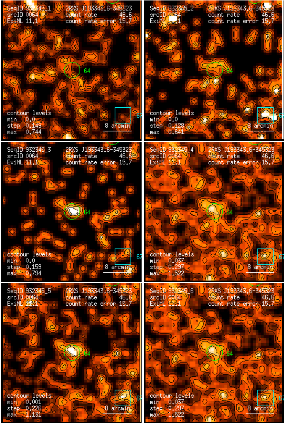
Figure 64: RASS 932345: detection 0064: band rate images, Gaussian filter: (1) PSPC channels 11 – 41, (2) 52 – 90, (3) 91 – 201, (4) 11 – 235, (5) 52 – 201, (6) 11 – 201. Broad band rates in counts/ks. Band rate contour levels in counts/ks/arcmin 2 .
