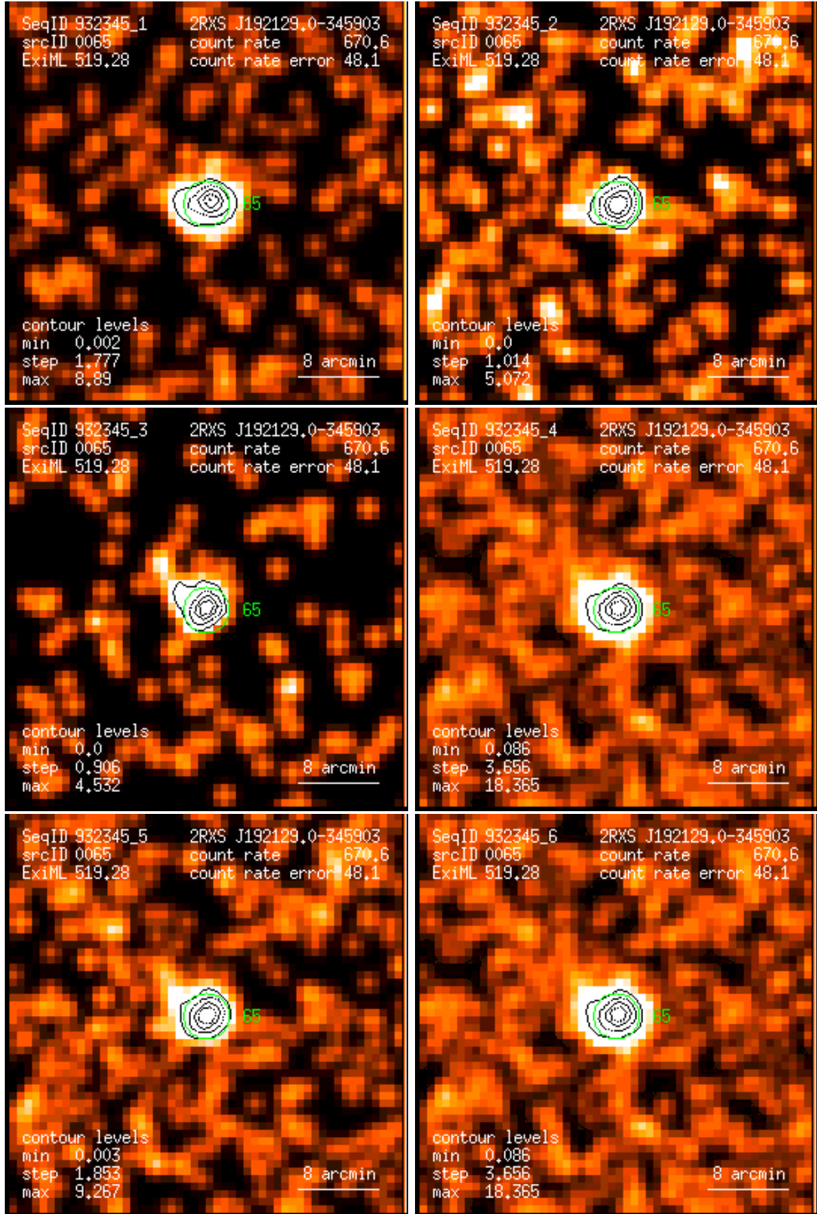
Figure 65: RASS 932345: detection 0065: band rate images, Gaussian filter: (1) PSPC channels 11 – 41, (2) 52 – 90, (3) 91 – 201, (4) 11 – 235, (5) 52 – 201, (6) 11 – 201. Broad band rates in counts/ks. Band rate contour levels in counts/ks/arcmin 2 .
