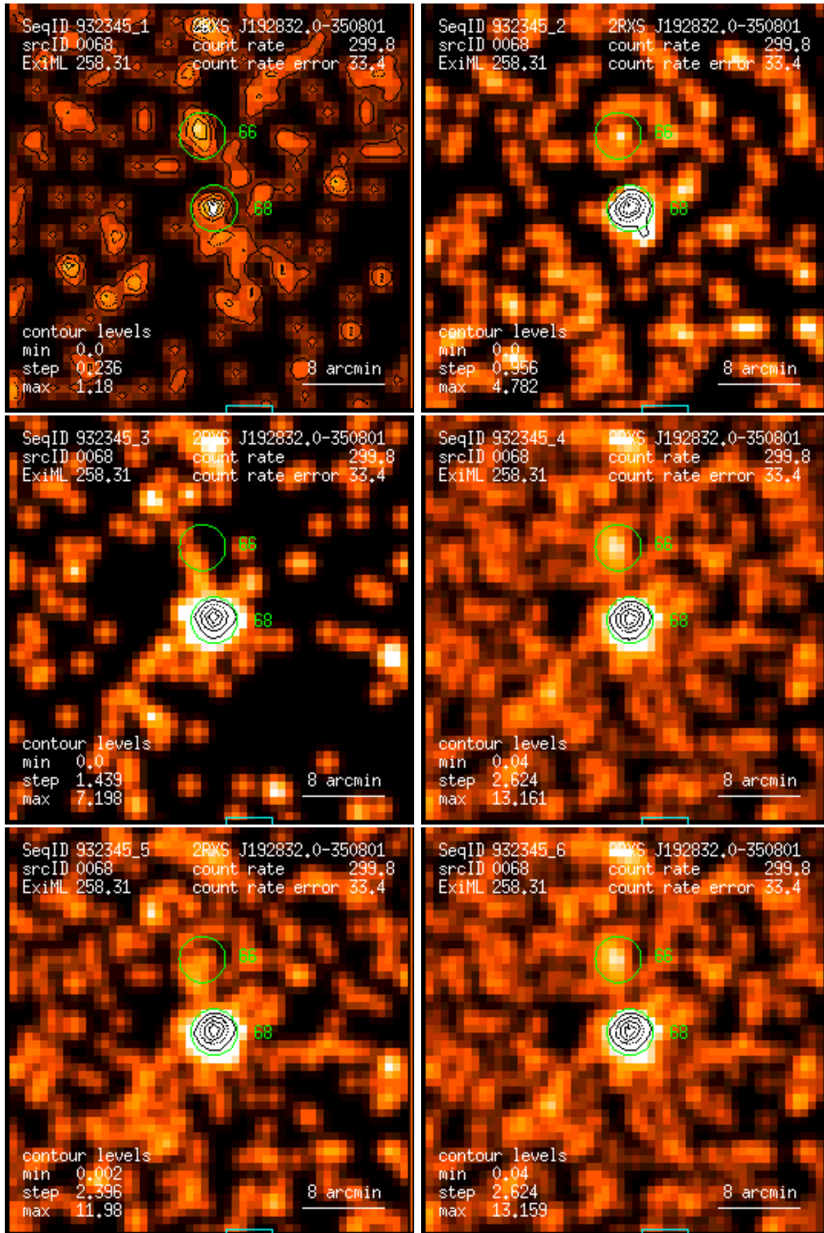
Figure 68: RASS 932345: detection 0068: band rate images, Gaussian filter: (1) PSPC channels 11 – 41, (2) 52 – 90, (3) 91 – 201, (4) 11 – 235, (5) 52 – 201, (6) 11 – 201. Broad band rates in counts/ks. Band rate contour levels in counts/ks/arcmin 2 .
