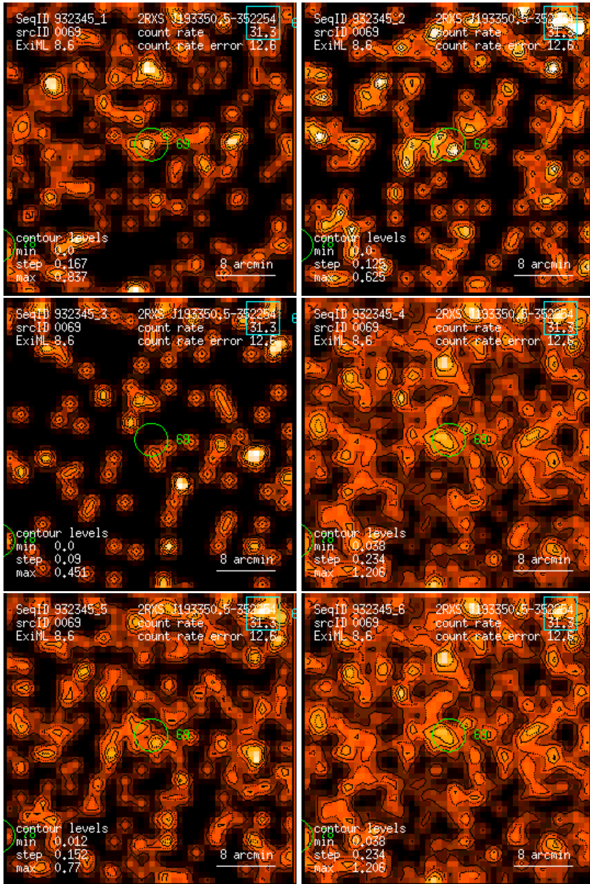
Figure 69: RASS 932345: detection 0069: band rate images, Gaussian filter: (1) PSPC channels 11 – 41, (2) 52 – 90, (3) 91 – 201, (4) 11 – 235, (5) 52 – 201, (6) 11 – 201. Broad band rates in counts/ks. Band rate contour levels in counts/ks/arcmin 2 .
