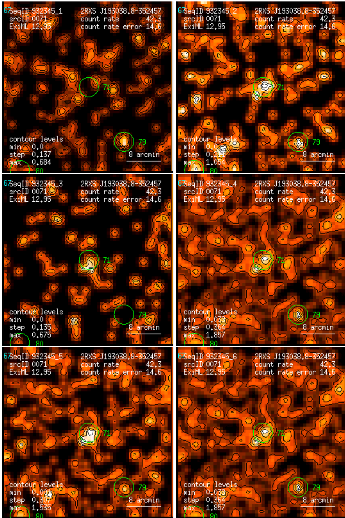
Figure 71: RASS 932345: detection 0071: band rate images, Gaussian filter: (1) PSPC channels 11 – 41, (2) 52 – 90, (3) 91 – 201, (4) 11 – 235, (5) 52 – 201, (6) 11 – 201. Broad band rates in counts/ks. Band rate contour levels in counts/ks/arcmin 2 .
