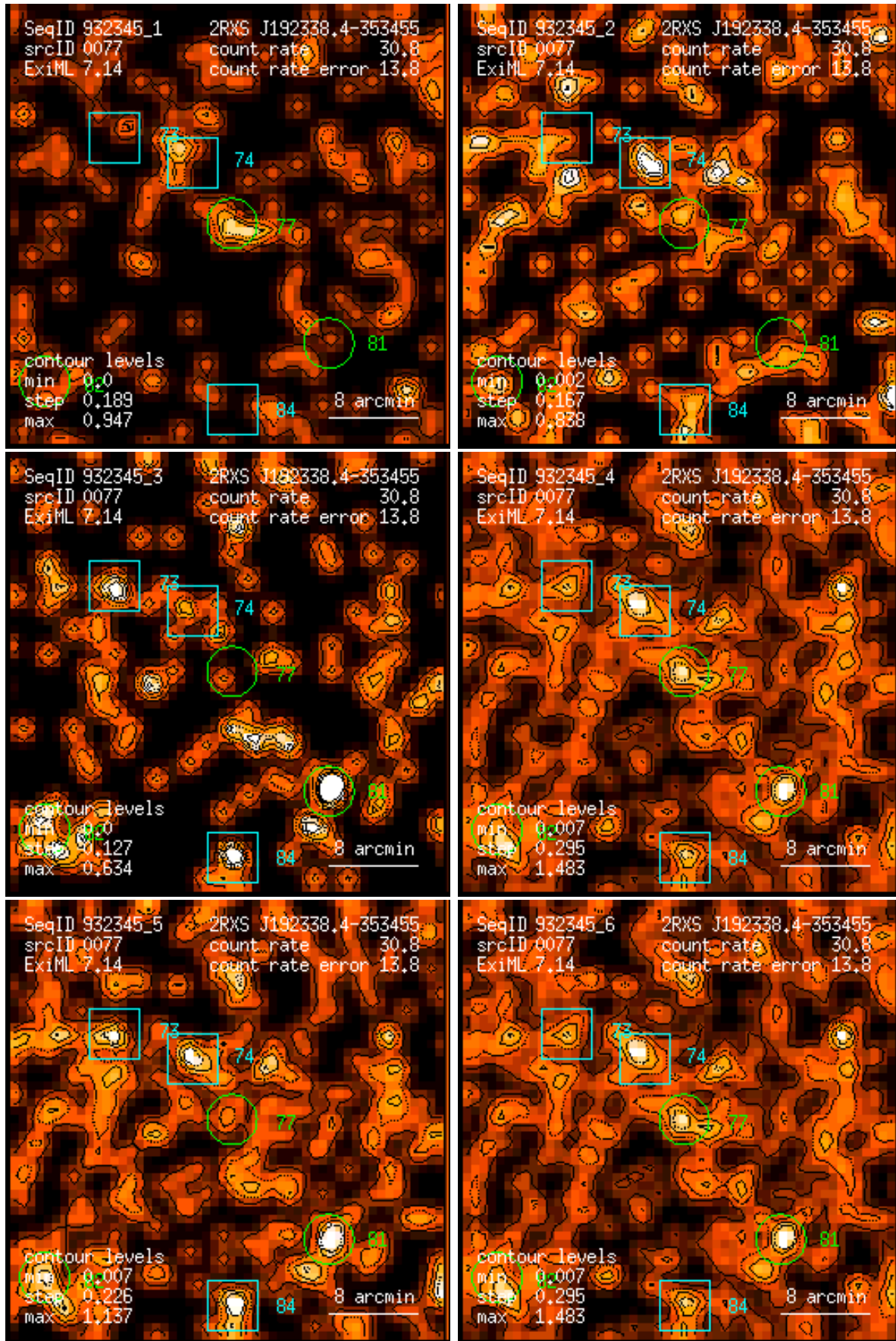
Figure 77: RASS 932345: detection 0077: band rate images, Gaussian filter: (1) PSPC channels 11 – 41, (2) 52 – 90, (3) 91 – 201, (4) 11 – 235, (5) 52 – 201, (6) 11 – 201. Broad band rates in counts/ks. Band rate contour levels in counts/ks/arcmin 2 .
