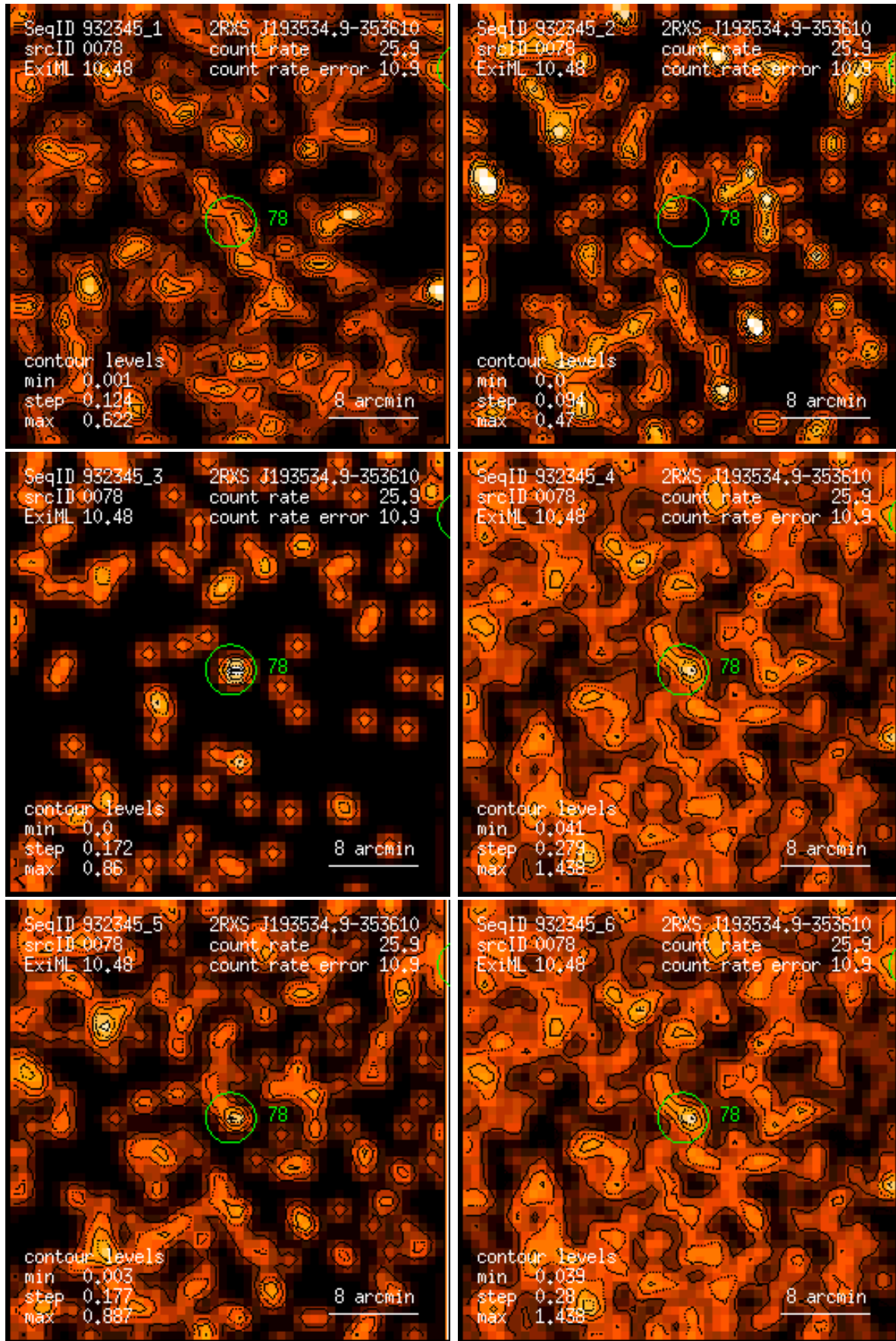
Figure 78: RASS 932345: detection 0078: band rate images, Gaussian filter: (1) PSPC channels 11 – 41, (2) 52 – 90, (3) 91 – 201, (4) 11 – 235, (5) 52 – 201, (6) 11 – 201. Broad band rates in counts/ks. Band rate contour levels in counts/ks/arcmin 2 .
