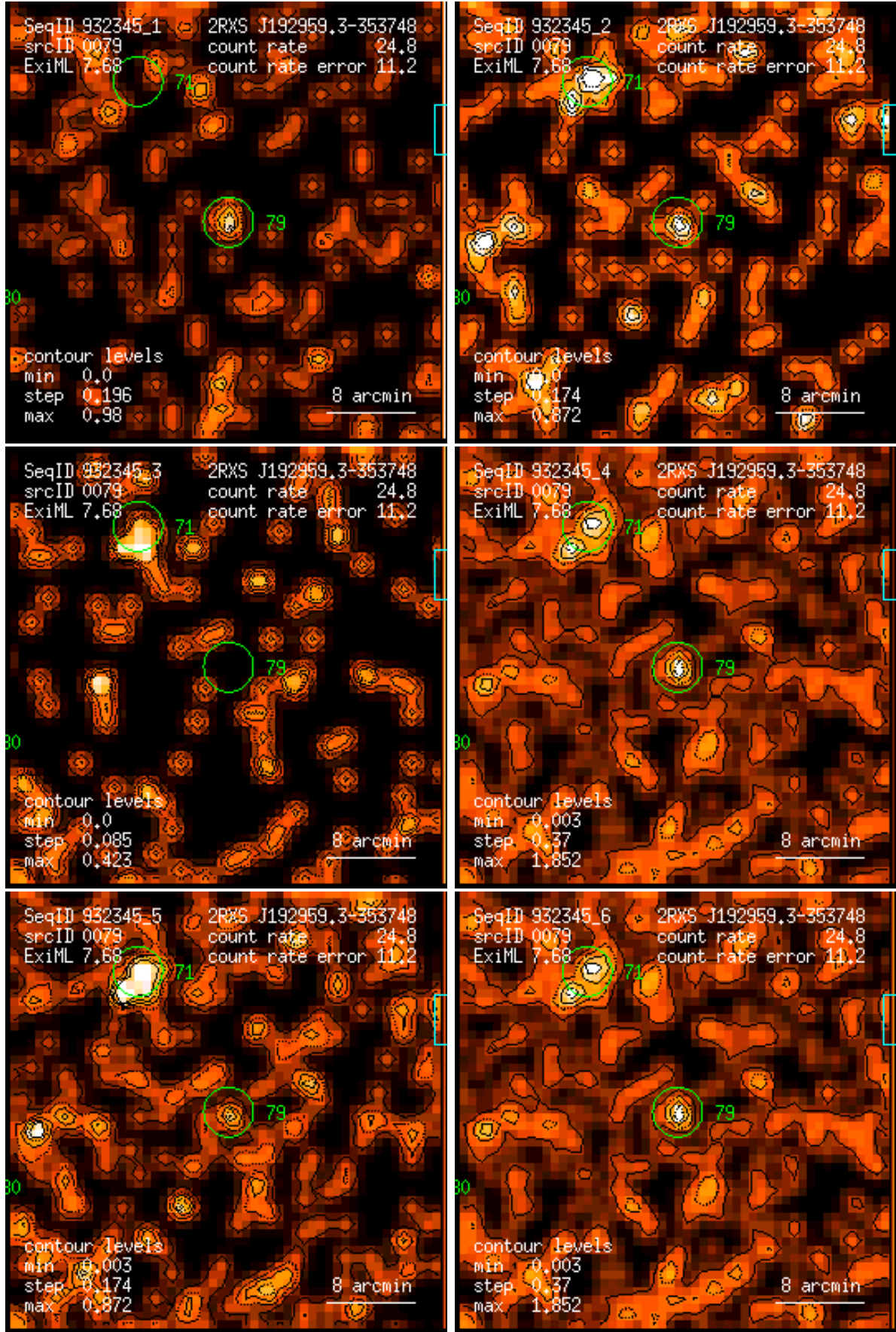
Figure 79: RASS 932345: detection 0079: band rate images, Gaussian filter: (1) PSPC channels 11 – 41, (2) 52 – 90, (3) 91 – 201, (4) 11 – 235, (5) 52 – 201, (6) 11 – 201. Broad band rates in counts/ks. Band rate contour levels in counts/ks/arcmin 2 .
