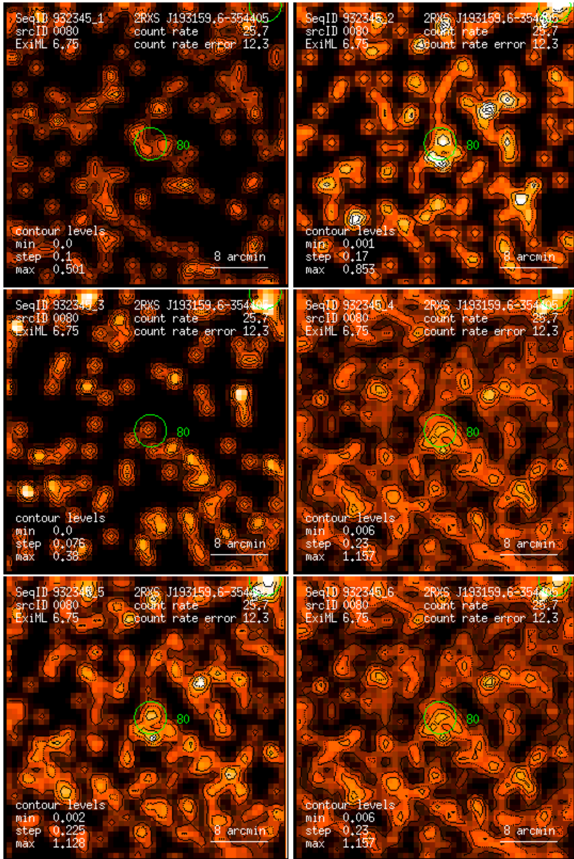
Figure 80: RASS 932345: detection 0080: band rate images, Gaussian filter: (1) PSPC channels 11 – 41, (2) 52 – 90, (3) 91 – 201, (4) 11 – 235, (5) 52 – 201, (6) 11 – 201. Broad band rates in counts/ks. Band rate contour levels in counts/ks/arcmin 2 .
