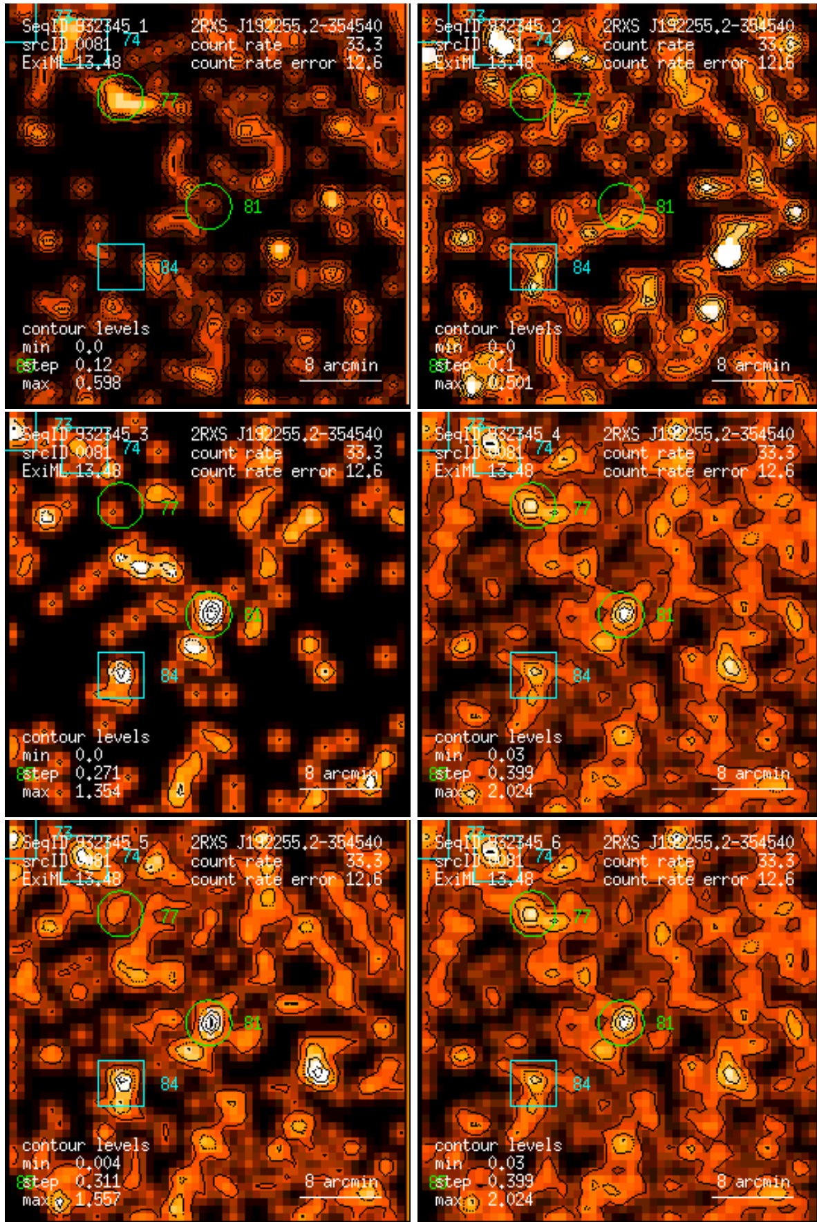
Figure 81: RASS 932345: detection 0081: band rate images, Gaussian filter: (1) PSPC channels 11 – 41, (2) 52 – 90, (3) 91 – 201, (4) 11 – 235, (5) 52 – 201, (6) 11 – 201. Broad band rates in counts/ks. Band rate contour levels in counts/ks/arcmin 2 .
