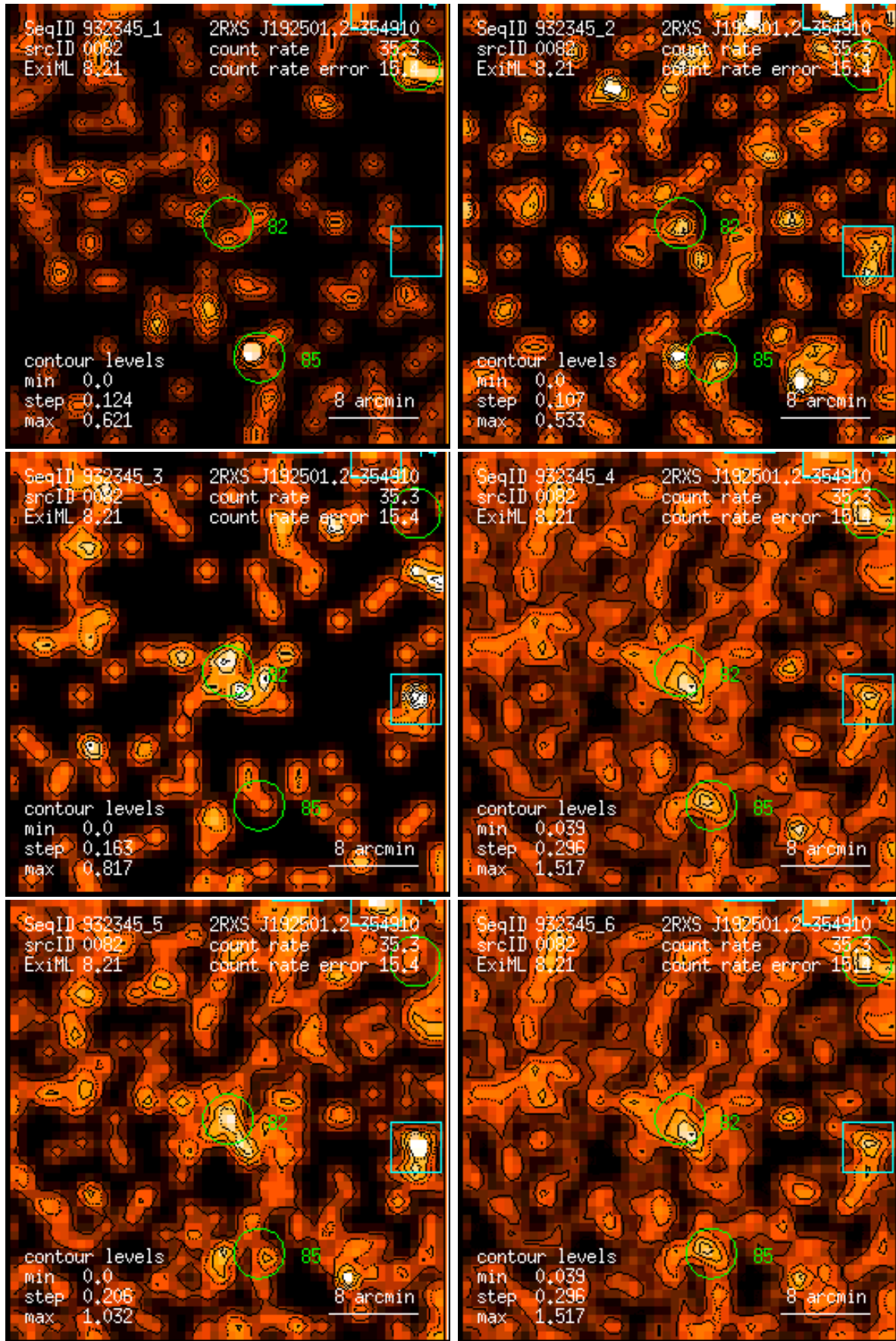
Figure 82: RASS 932345: detection 0082: band rate images, Gaussian filter: (1) PSPC channels 11 – 41, (2) 52 – 90, (3) 91 – 201, (4) 11 – 235, (5) 52 – 201, (6) 11 – 201. Broad band rates in counts/ks. Band rate contour levels in counts/ks/arcmin 2 .
