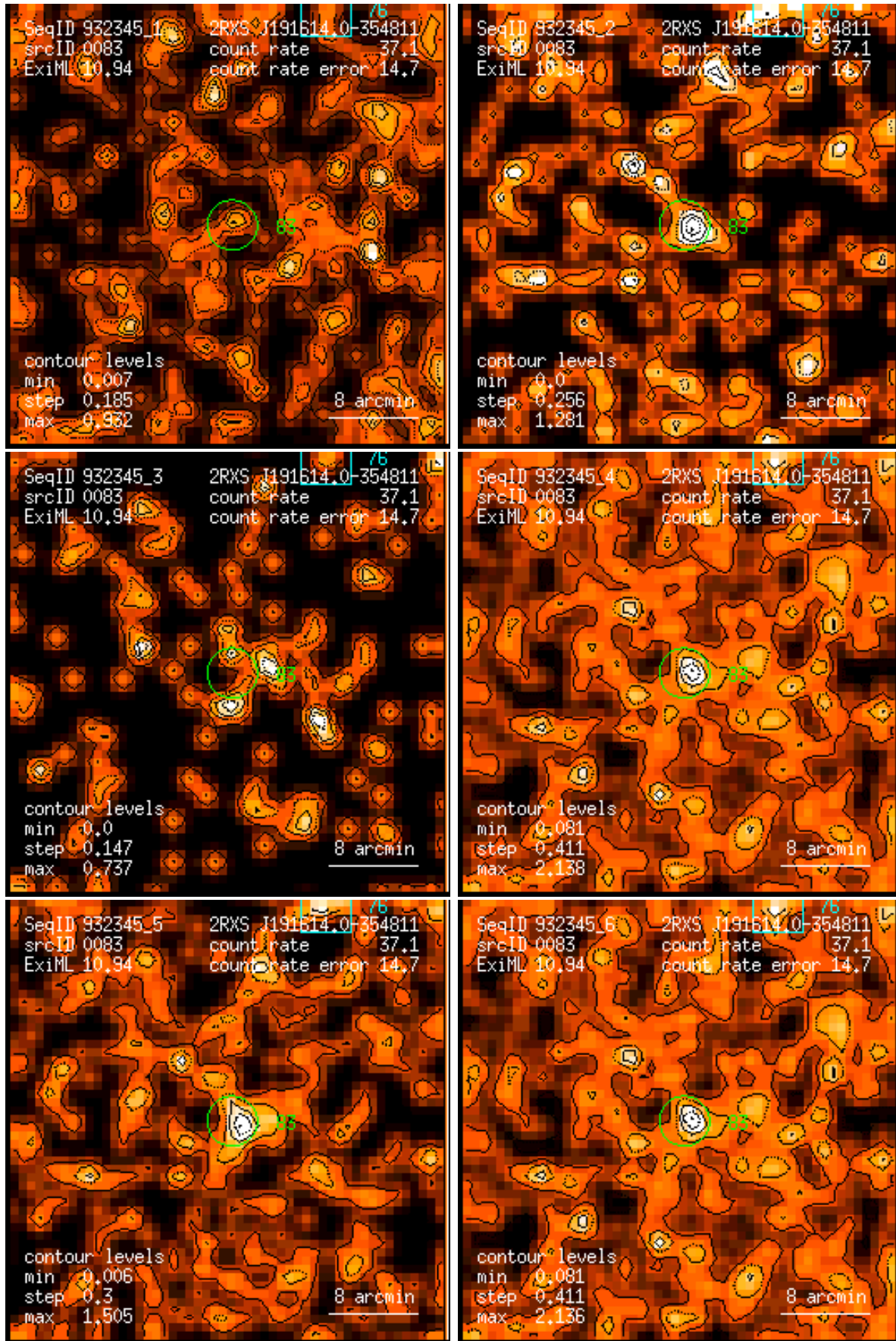
Figure 83: RASS 932345: detection 0083: band rate images, Gaussian filter: (1) PSPC channels 11 – 41, (2) 52 – 90, (3) 91 – 201, (4) 11 – 235, (5) 52 – 201, (6) 11 – 201. Broad band rates in counts/ks. Band rate contour levels in counts/ks/arcmin 2 .
