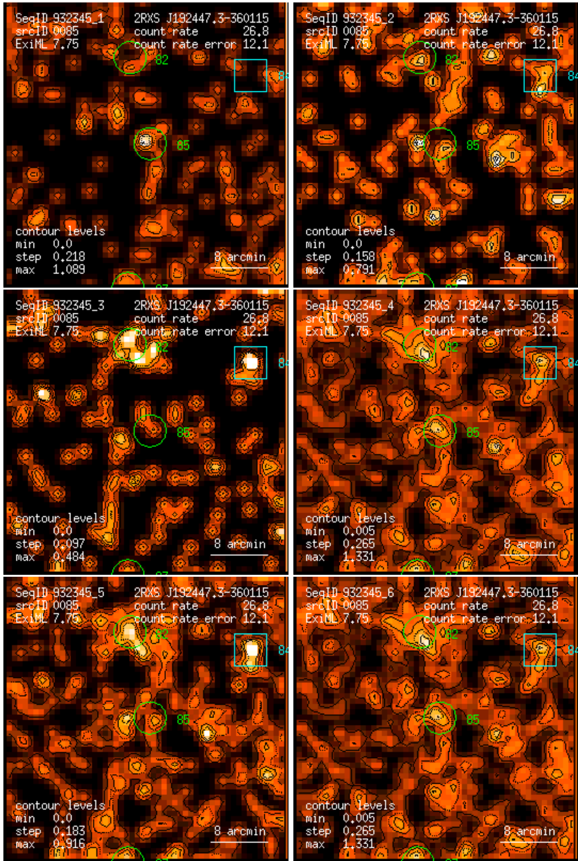
Figure 85: RASS 932345: detection 0085: band rate images, Gaussian filter: (1) PSPC channels 11 – 41, (2) 52 – 90, (3) 91 – 201, (4) 11 – 235, (5) 52 – 201, (6) 11 – 201. Broad band rates in counts/ks. Band rate contour levels in counts/ks/arcmin 2 .
