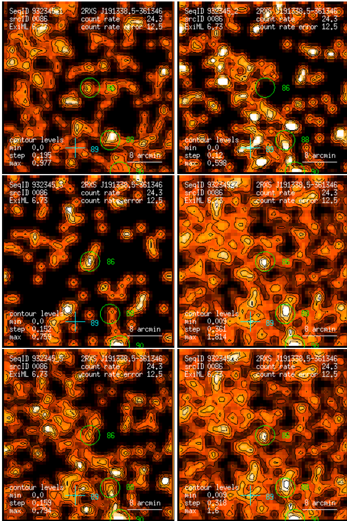
Figure 86: RASS 932345: detection 0086: band rate images, Gaussian filter: (1) PSPC channels 11 – 41, (2) 52 – 90, (3) 91 – 201, (4) 11 – 235, (5) 52 – 201, (6) 11 – 201. Broad band rates in counts/ks. Band rate contour levels in counts/ks/arcmin 2 .
