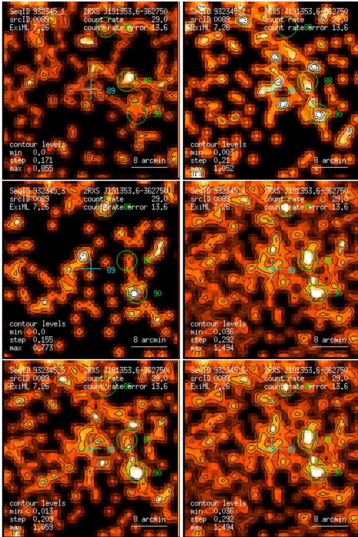
Figure 89: RASS 932345: detection 0089: band rate images, Gaussian filter: (1) PSPC channels 11 – 41, (2) 52 – 90, (3) 91 – 201, (4) 11 – 235, (5) 52 – 201, (6) 11 – 201. Broad band rates in counts/ks. Band rate contour levels in counts/ks/arcmin 2 .
