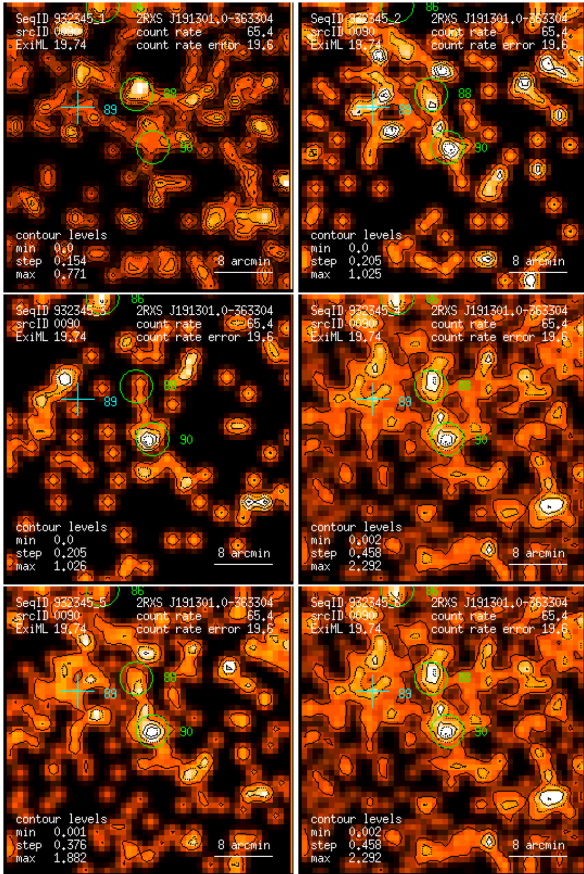
Figure 90: RASS 932345: detection 0090: band rate images, Gaussian filter: (1) PSPC channels 11 – 41, (2) 52 – 90, (3) 91 – 201, (4) 11 – 235, (5) 52 – 201, (6) 11 – 201. Broad band rates in counts/ks. Band rate contour levels in counts/ks/arcmin 2 .
