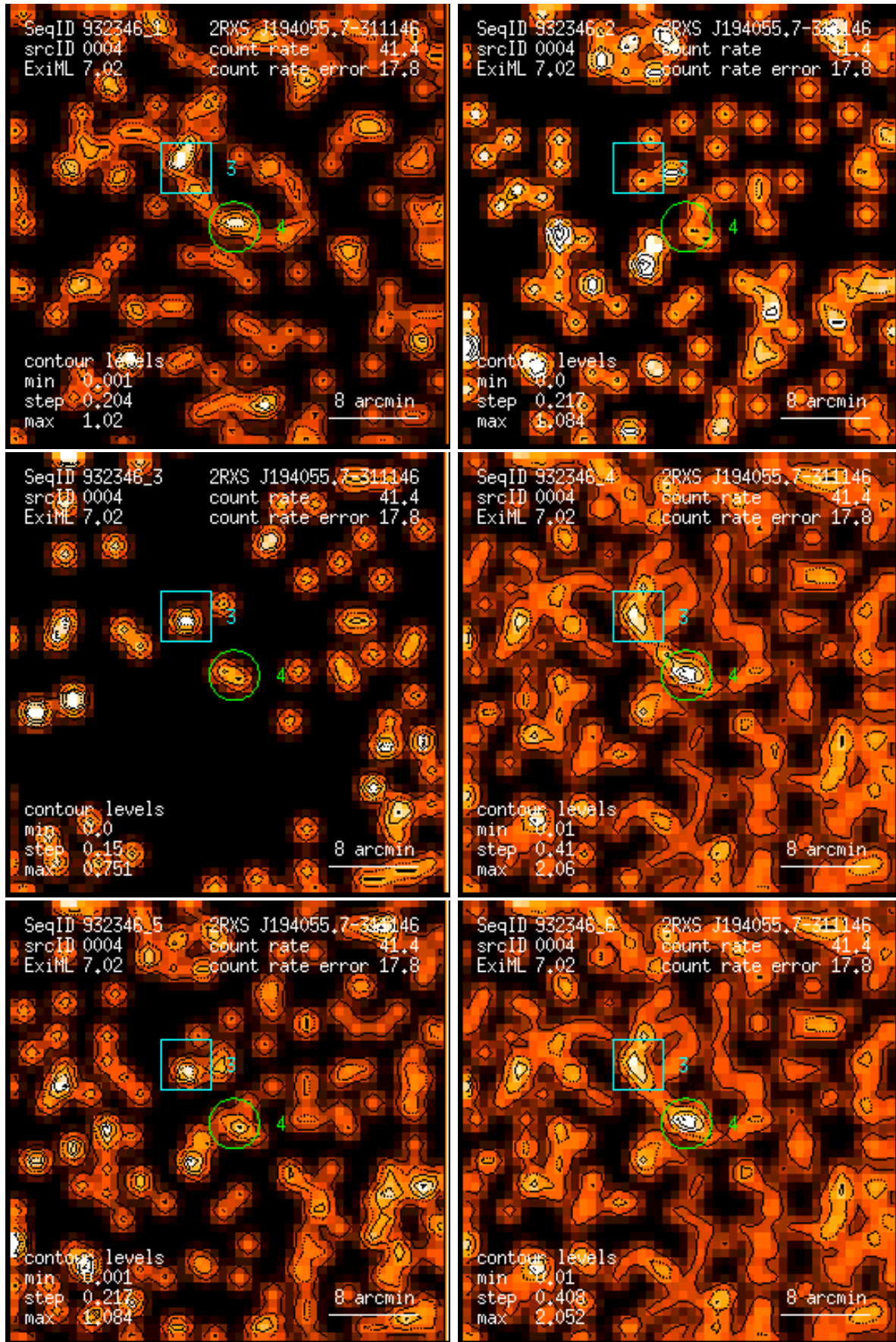
Figure 4: RASS 932346: detection 0004: band rate images, Gaussian filter: (1) PSPC channels 11 – 41, (2) 52 – 90, (3) 91 – 201, (4) 11 – 235, (5) 52 – 201, (6) 11 – 201. Broad band rates in counts/ks. Band rate contour levels in counts/ks/arcmin 2 .
