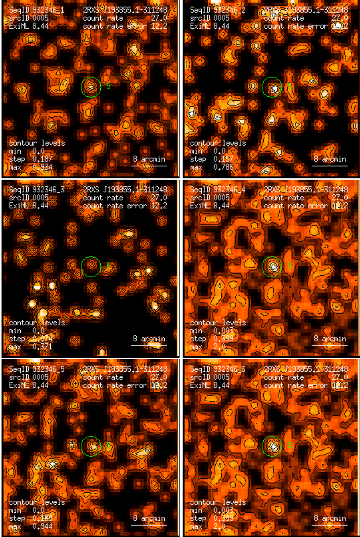
Figure 5: RASS 932346: detection 0005: band rate images, Gaussian filter: (1) PSPC channels 11 – 41, (2) 52 – 90, (3) 91 – 201, (4) 11 – 235, (5) 52 – 201, (6) 11 – 201. Broad band rates in counts/ks. Band rate contour levels in counts/ks/arcmin 2 .
