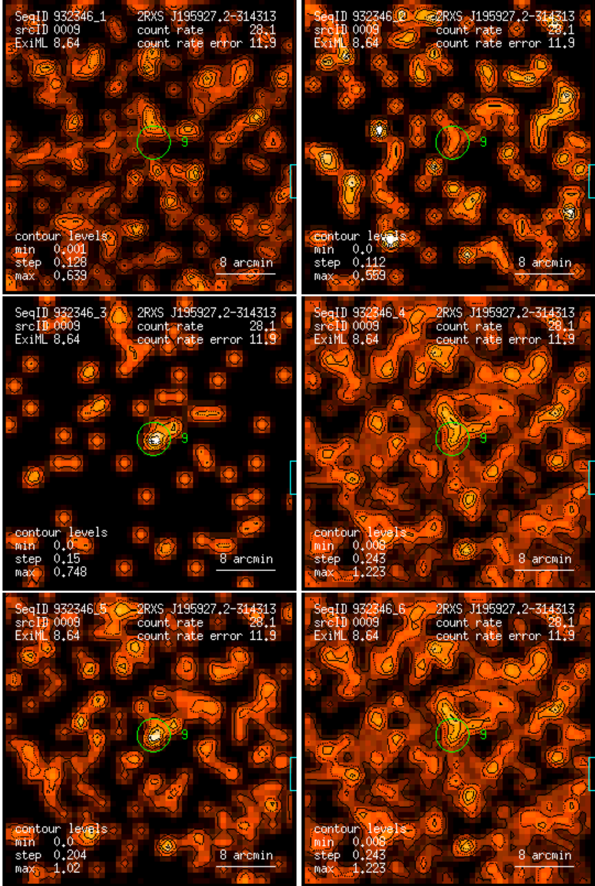
Figure 9: RASS 932346: detection 0009: band rate images, Gaussian filter: (1) PSPC channels 11 – 41, (2) 52 – 90, (3) 91 – 201, (4) 11 – 235, (5) 52 – 201, (6) 11 – 201. Broad band rates in counts/ks. Band rate contour levels in counts/ks/arcmin 2 .
