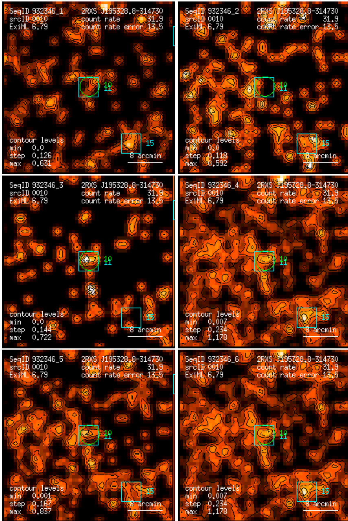
Figure 10: RASS 932346: detection 0010: band rate images, Gaussian filter: (1) PSPC channels 11 – 41, (2) 52 – 90, (3) 91 – 201, (4) 11 – 235, (5) 52 – 201, (6) 11 – 201. Broad band rates in counts/ks. Band rate contour levels in counts/ks/arcmin 2 .
