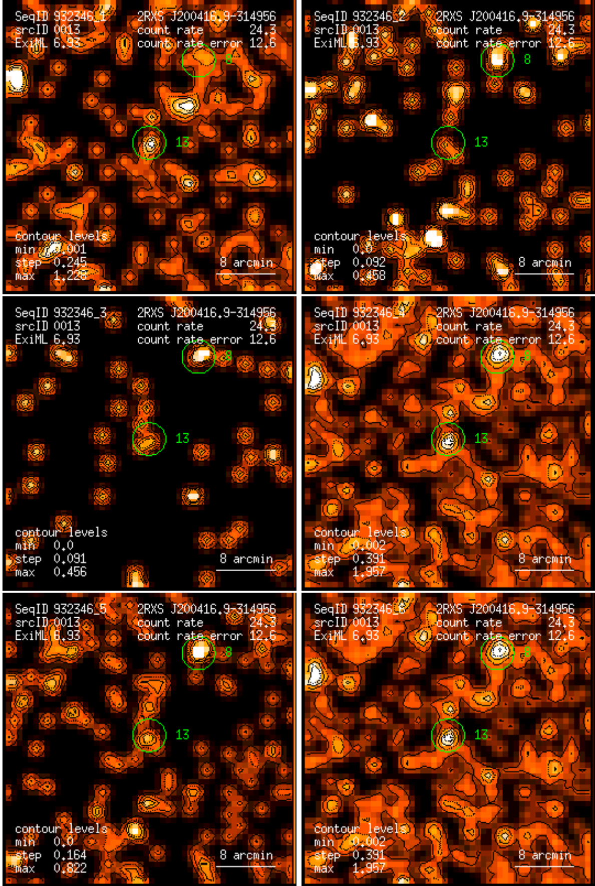
Figure 13: RASS 932346: detection 0013: band rate images, Gaussian filter: (1) PSPC channels 11 – 41, (2) 52 – 90, (3) 91 – 201, (4) 11 – 235, (5) 52 – 201, (6) 11 – 201. Broad band rates in counts/ks. Band rate contour levels in counts/ks/arcmin 2 .
