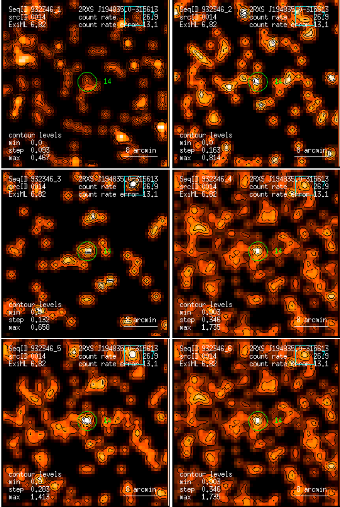
Figure 14: RASS 932346: detection 0014: band rate images, Gaussian filter: (1) PSPC channels 11 – 41, (2) 52 – 90, (3) 91 – 201, (4) 11 – 235, (5) 52 – 201, (6) 11 – 201. Broad band rates in counts/ks. Band rate contour levels in counts/ks/arcmin 2 .
