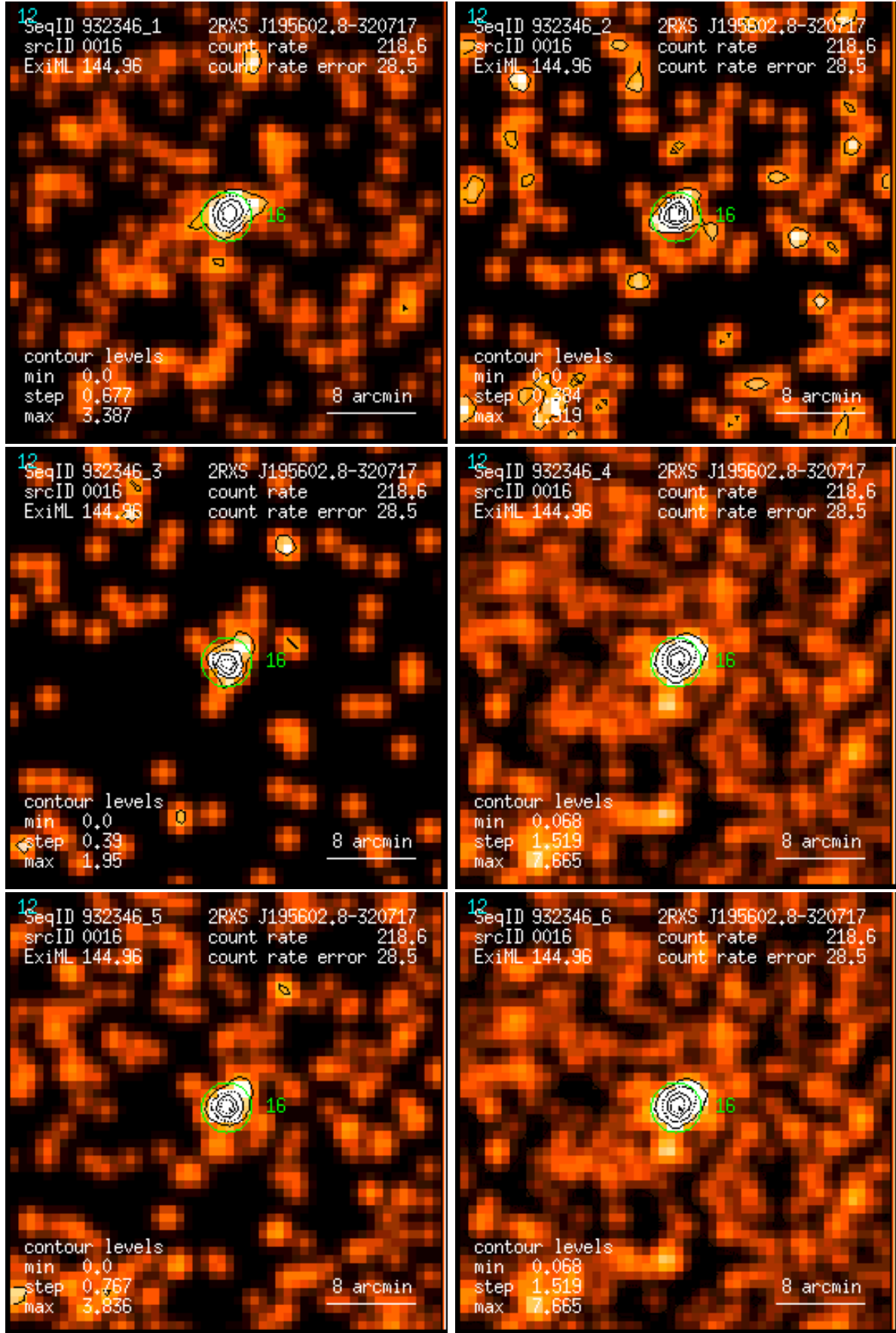
Figure 16: RASS 932346: detection 0016: band rate images, Gaussian filter: (1) PSPC channels 11 – 41, (2) 52 – 90, (3) 91 – 201, (4) 11 – 235, (5) 52 – 201, (6) 11 – 201. Broad band rates in counts/ks. Band rate contour levels in counts/ks/arcmin 2 .
