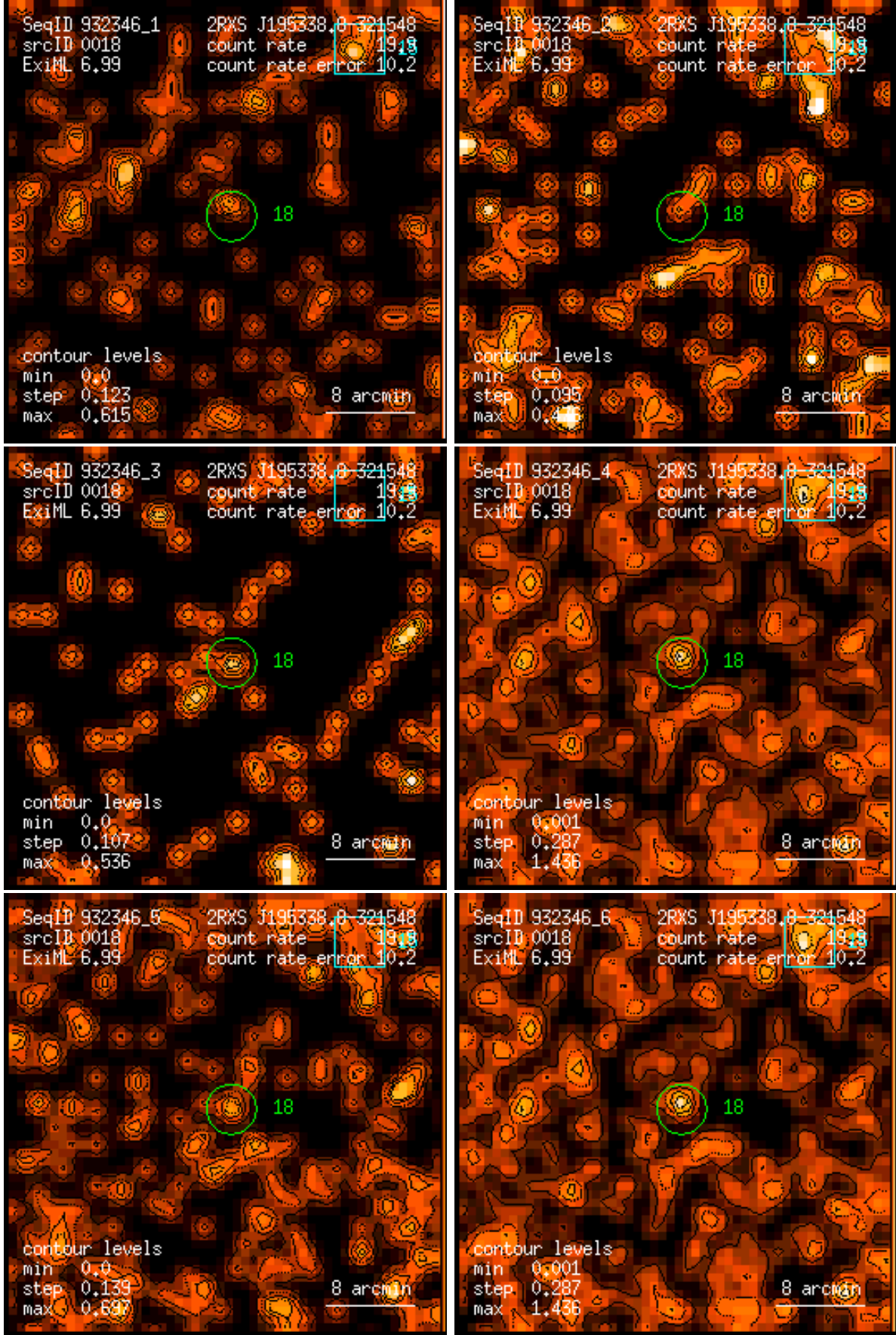
Figure 18: RASS 932346: detection 0018: band rate images, Gaussian filter: (1) PSPC channels 11 – 41, (2) 52 – 90, (3) 91 – 201, (4) 11 – 235, (5) 52 – 201, (6) 11 – 201. Broad band rates in counts/ks. Band rate contour levels in counts/ks/arcmin 2 .
