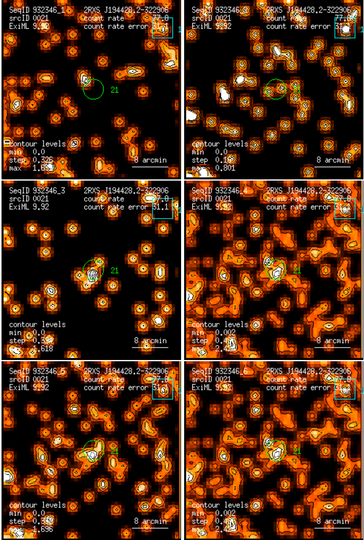
Figure 21: RASS 932346: detection 0021: band rate images, Gaussian filter: (1) PSPC channels 11 – 41, (2) 52 – 90, (3) 91 – 201, (4) 11 – 235, (5) 52 – 201, (6) 11 – 201. Broad band rates in counts/ks. Band rate contour levels in counts/ks/arcmin 2 .
