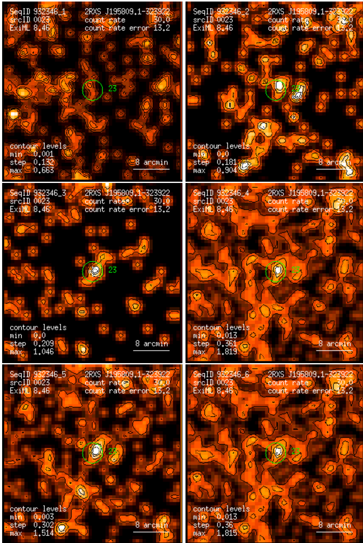
Figure 23: RASS 932346: detection 0023: band rate images, Gaussian filter: (1) PSPC channels 11 – 41, (2) 52 – 90, (3) 91 – 201, (4) 11 – 235, (5) 52 – 201, (6) 11 – 201. Broad band rates in counts/ks. Band rate contour levels in counts/ks/arcmin 2 .
