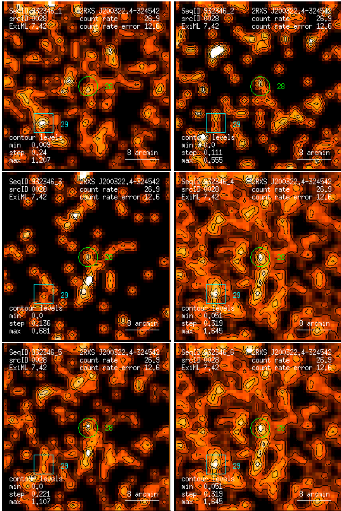
Figure 28: RASS 932346: detection 0028: band rate images, Gaussian filter: (1) PSPC channels 11 – 41, (2) 52 – 90, (3) 91 – 201, (4) 11 – 235, (5) 52 – 201, (6) 11 – 201. Broad band rates in counts/ks. Band rate contour levels in counts/ks/arcmin 2 .
