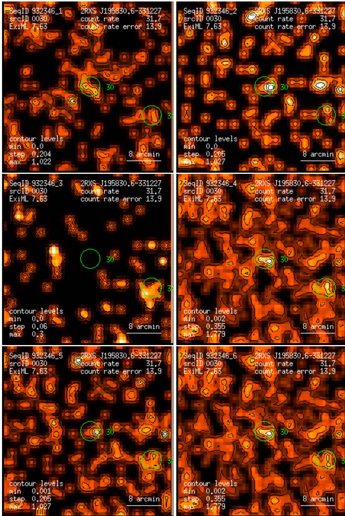
Figure 30: RASS 932346: detection 0030: band rate images, Gaussian filter: (1) PSPC channels 11 – 41, (2) 52 – 90, (3) 91 – 201, (4) 11 – 235, (5) 52 – 201, (6) 11 – 201. Broad band rates in counts/ks. Band rate contour levels in counts/ks/arcmin 2 .
