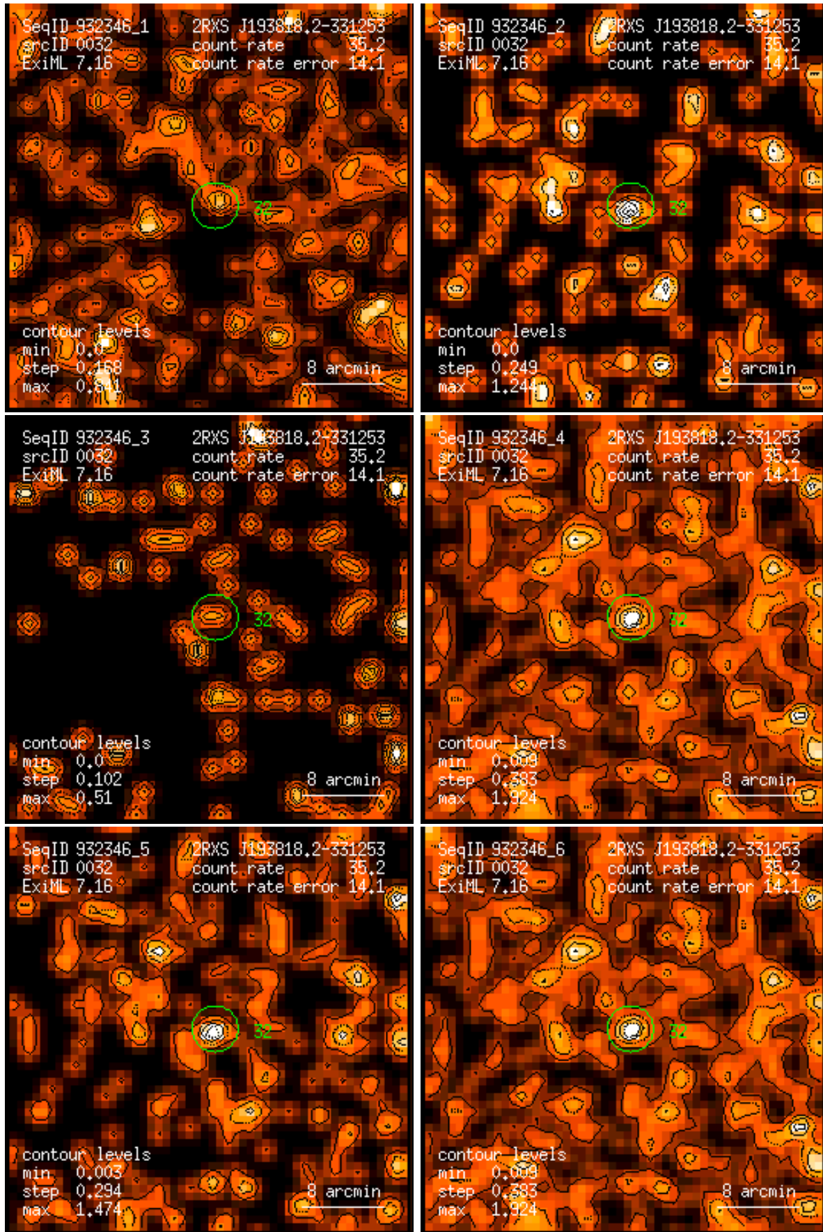
Figure 32: RASS 932346: detection 0032: band rate images, Gaussian filter: (1) PSPC channels 11 – 41, (2) 52 – 90, (3) 91 – 201, (4) 11 – 235, (5) 52 – 201, (6) 11 – 201. Broad band rates in counts/ks. Band rate contour levels in counts/ks/arcmin 2 .
